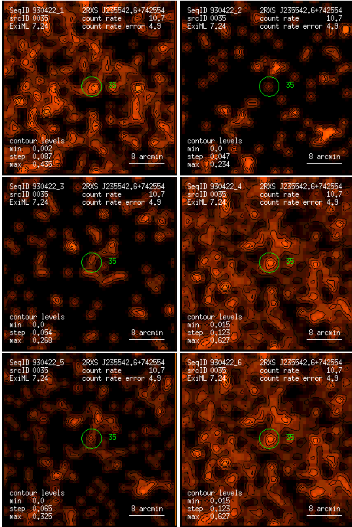
Figure 35: RASS 930422: detection 0035: band rate images, Gaussian filter: (1) PSPC channels 11 – 41, (2) 52 – 90, (3) 91 – 201, (4) 11 – 235, (5) 52 – 201, (6) 11 – 201. Broad band rates in counts/ks. Band rate contour levels in counts/ks/arcmin 2 .
