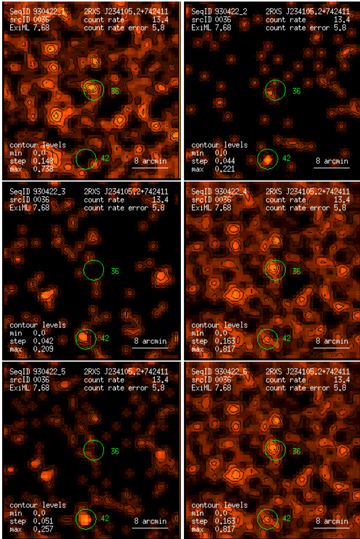
Figure 36: RASS 930422: detection 0036: band rate images, Gaussian filter: (1) PSPC channels 11 – 41, (2) 52 – 90, (3) 91 – 201, (4) 11 – 235, (5) 52 – 201, (6) 11 – 201. Broad band rates in counts/ks. Band rate contour levels in counts/ks/arcmin 2 .
