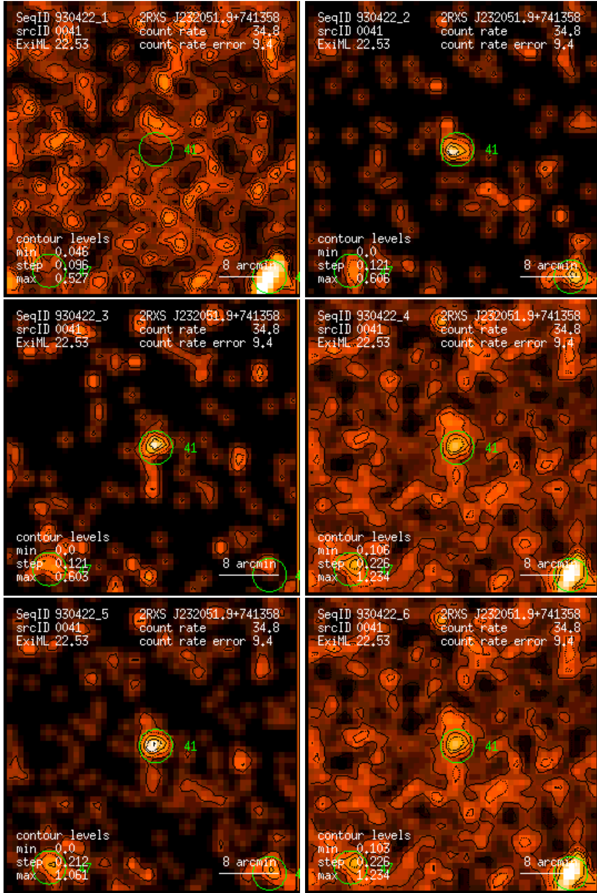
Figure 41: RASS 930422: detection 0041: band rate images, Gaussian filter: (1) PSPC channels 11 – 41, (2) 52 – 90, (3) 91 – 201, (4) 11 – 235, (5) 52 – 201, (6) 11 – 201. Broad band rates in counts/ks. Band rate contour levels in counts/ks/arcmin 2 .
