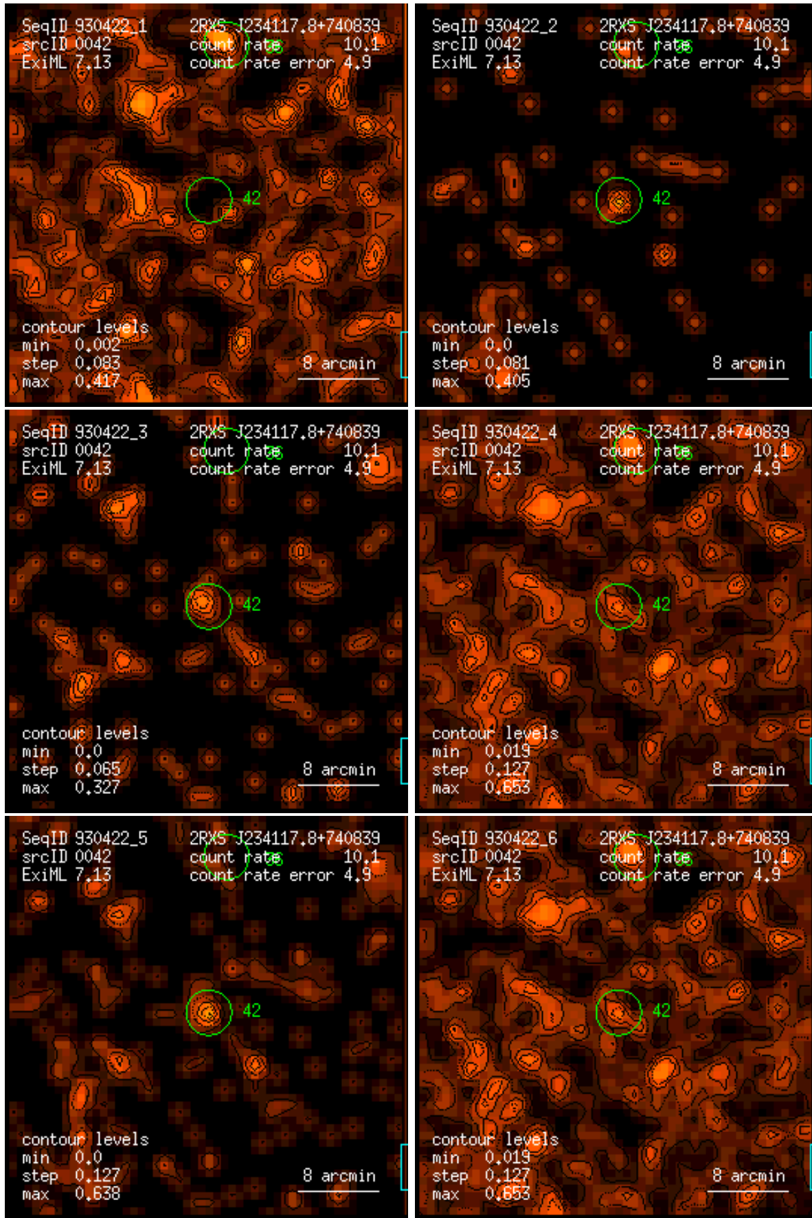
Figure 42: RASS 930422: detection 0042: band rate images, Gaussian filter: (1) PSPC channels 11 – 41, (2) 52 – 90, (3) 91 – 201, (4) 11 – 235, (5) 52 – 201, (6) 11 – 201. Broad band rates in counts/ks. Band rate contour levels in counts/ks/arcmin 2 .
