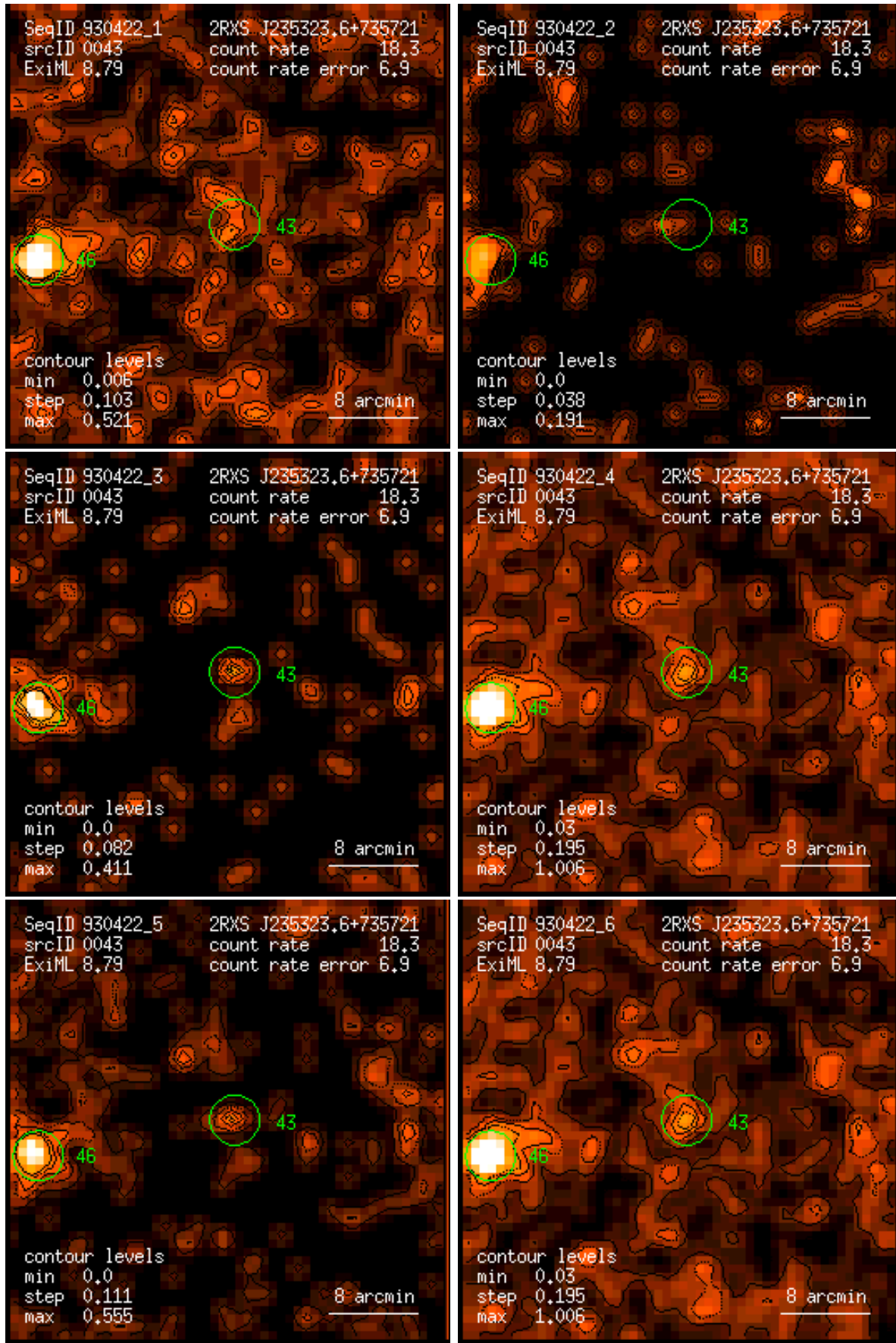
Figure 43: RASS 930422: detection 0043: band rate images, Gaussian filter: (1) PSPC channels 11 – 41, (2) 52 – 90, (3) 91 – 201, (4) 11 – 235, (5) 52 – 201, (6) 11 – 201. Broad band rates in counts/ks. Band rate contour levels in counts/ks/arcmin 2 .
