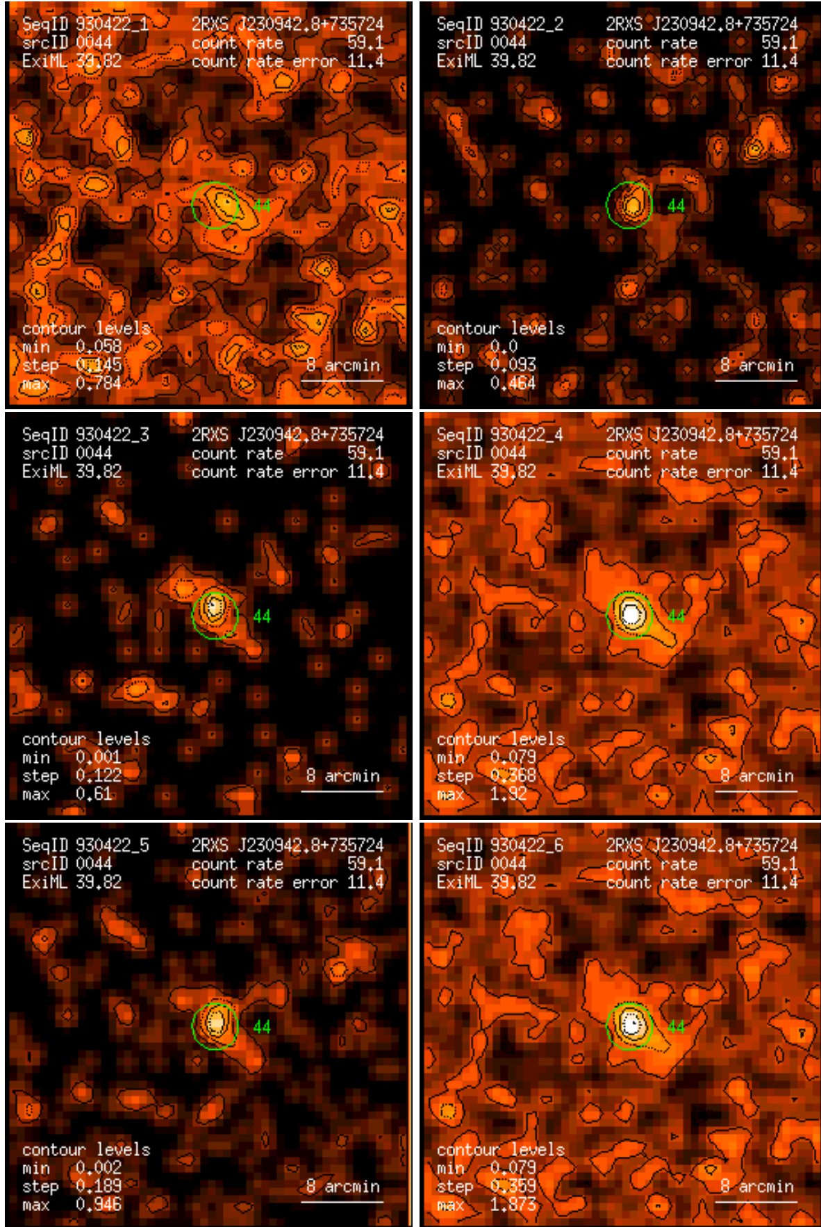
Figure 44: RASS 930422: detection 0044: band rate images, Gaussian filter: (1) PSPC channels 11 – 41, (2) 52 – 90, (3) 91 – 201, (4) 11 – 235, (5) 52 – 201, (6) 11 – 201. Broad band rates in counts/ks. Band rate contour levels in counts/ks/arcmin 2 .
