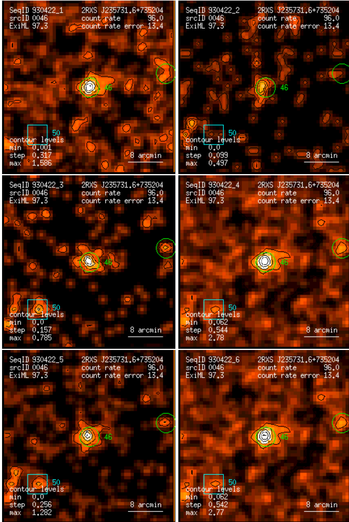
Figure 46: RASS 930422: detection 0046: band rate images, Gaussian filter: (1) PSPC channels 11 – 41, (2) 52 – 90, (3) 91 – 201, (4) 11 – 235, (5) 52 – 201, (6) 11 – 201. Broad band rates in counts/ks. Band rate contour levels in counts/ks/arcmin 2 .
