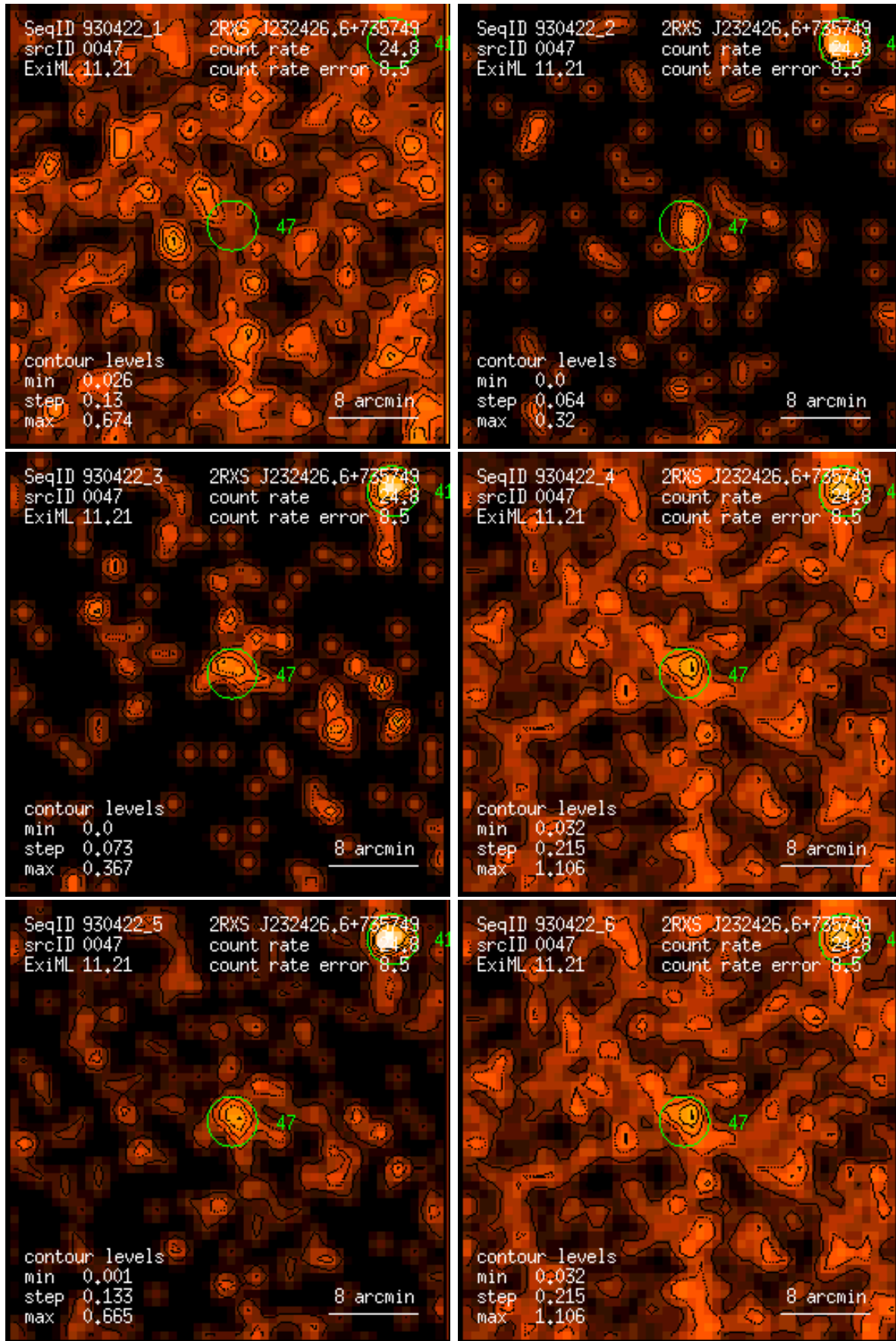
Figure 47: RASS 930422: detection 0047: band rate images, Gaussian filter: (1) PSPC channels 11 – 41, (2) 52 – 90, (3) 91 – 201, (4) 11 – 235, (5) 52 – 201, (6) 11 – 201. Broad band rates in counts/ks. Band rate contour levels in counts/ks/arcmin 2 .
