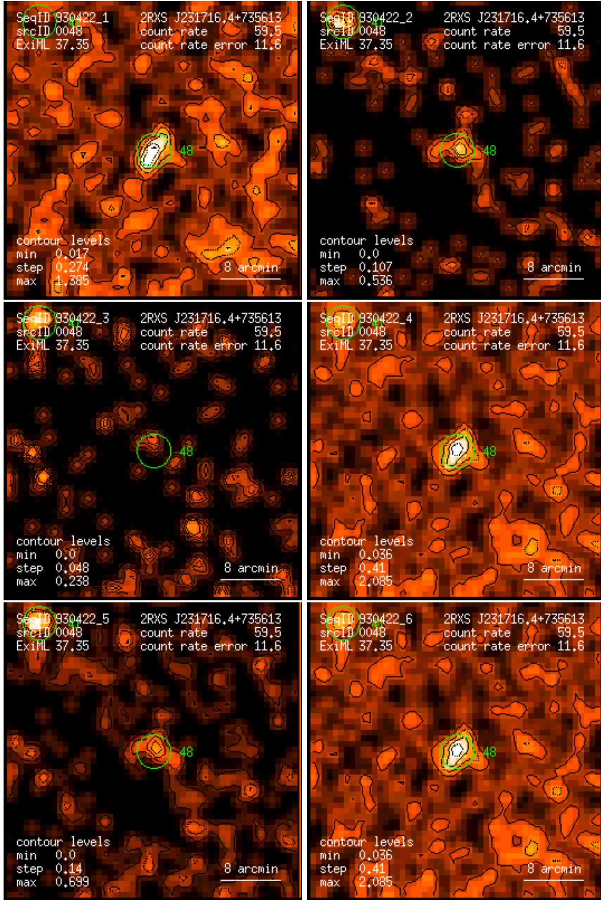
Figure 48: RASS 930422: detection 0048: band rate images, Gaussian filter: (1) PSPC channels 11 – 41, (2) 52 – 90, (3) 91 – 201, (4) 11 – 235, (5) 52 – 201, (6) 11 – 201. Broad band rates in counts/ks. Band rate contour levels in counts/ks/arcmin 2 .
