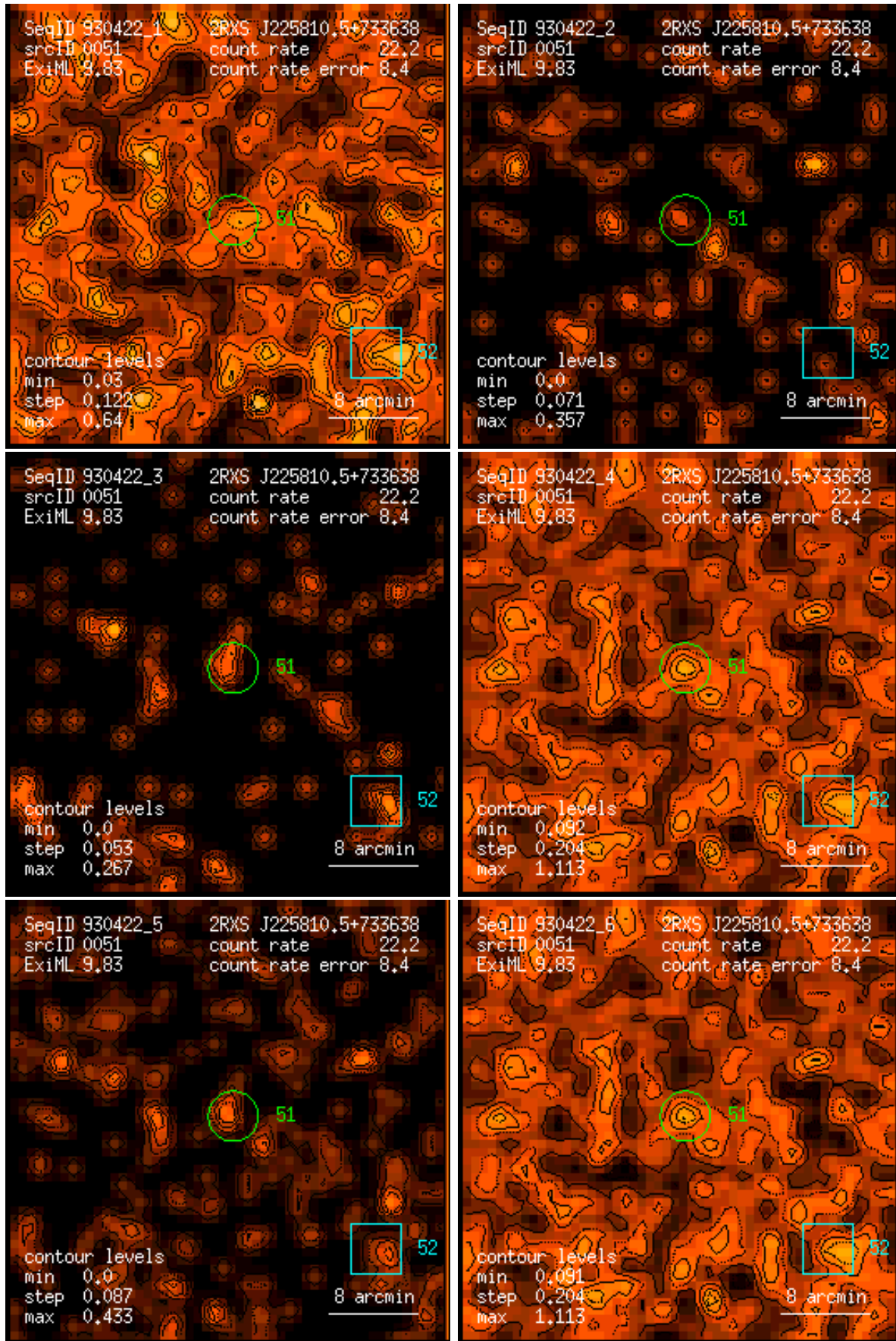
Figure 51: RASS 930422: detection 0051: band rate images, Gaussian filter: (1) PSPC channels 11 – 41, (2) 52 – 90, (3) 91 – 201, (4) 11 – 235, (5) 52 – 201, (6) 11 – 201. Broad band rates in counts/ks. Band rate contour levels in counts/ks/arcmin 2 .
