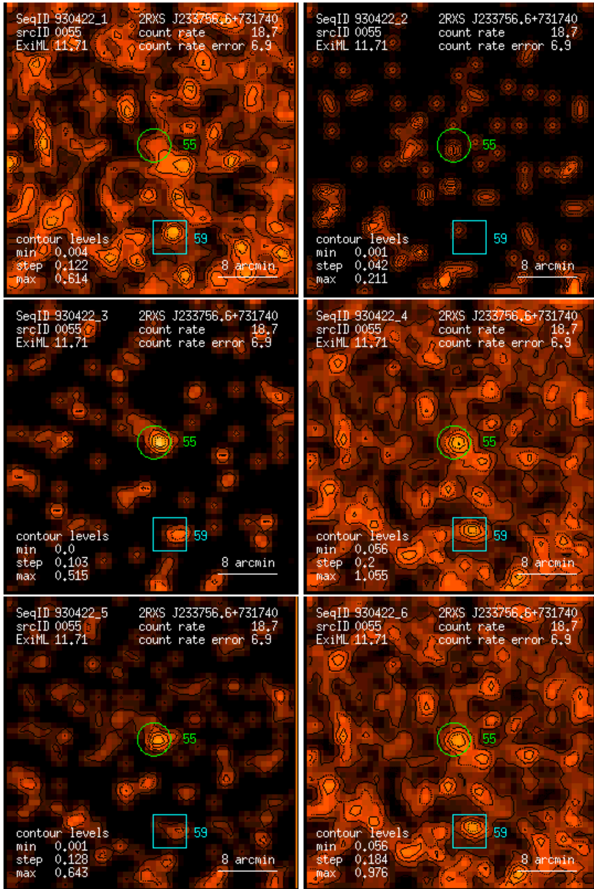
Figure 55: RASS 930422: detection 0055: band rate images, Gaussian filter: (1) PSPC channels 11 – 41, (2) 52 – 90, (3) 91 – 201, (4) 11 – 235, (5) 52 – 201, (6) 11 – 201. Broad band rates in counts/ks. Band rate contour levels in counts/ks/arcmin 2 .
