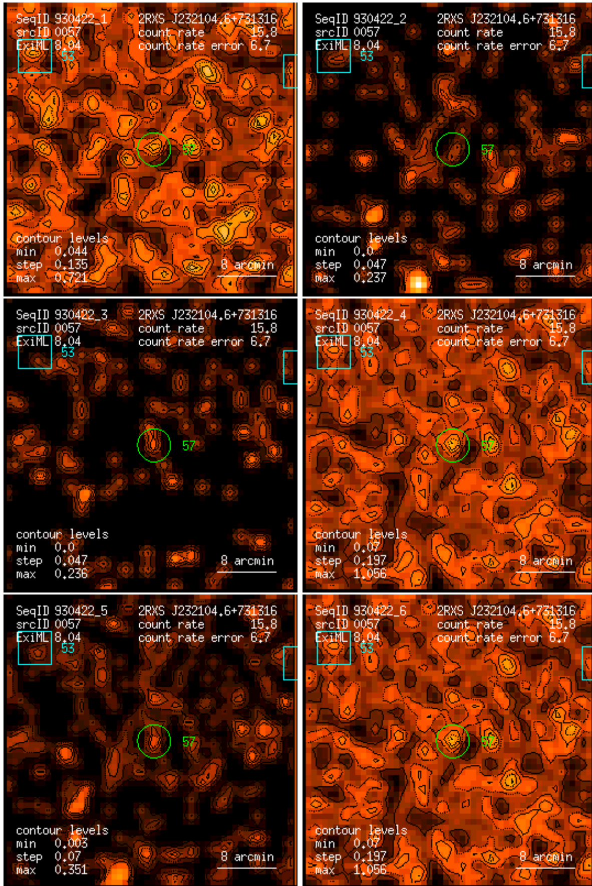
Figure 57: RASS 930422: detection 0057: band rate images, Gaussian filter: (1) PSPC channels 11 – 41, (2) 52 – 90, (3) 91 – 201, (4) 11 – 235, (5) 52 – 201, (6) 11 – 201. Broad band rates in counts/ks. Band rate contour levels in counts/ks/arcmin 2 .
