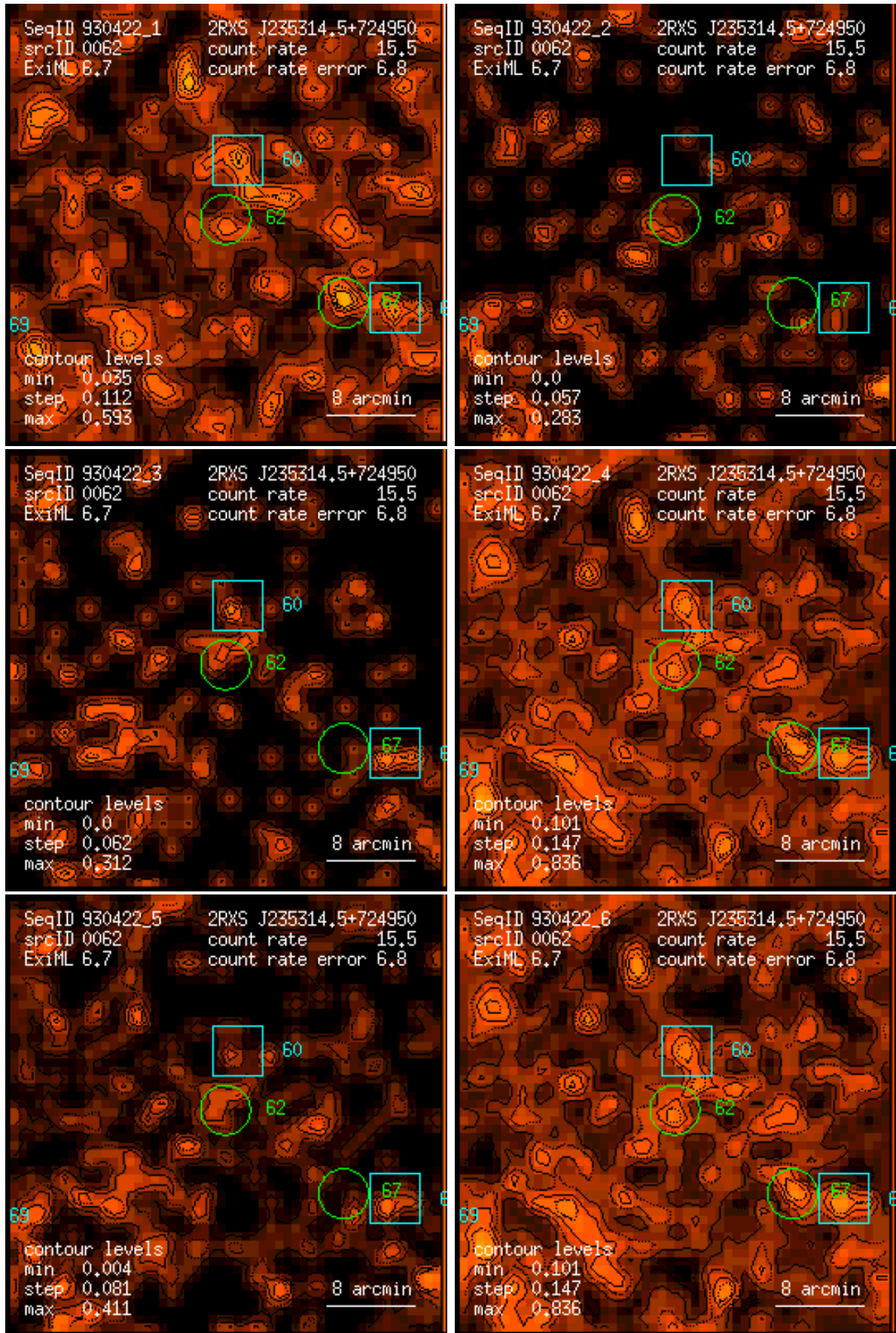
Figure 62: RASS 930422: detection 0062: band rate images, Gaussian filter: (1) PSPC channels 11 – 41, (2) 52 – 90, (3) 91 – 201, (4) 11 – 235, (5) 52 – 201, (6) 11 – 201. Broad band rates in counts/ks. Band rate contour levels in counts/ks/arcmin 2 .
