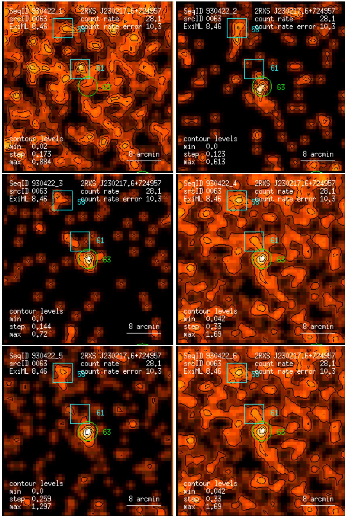
Figure 63: RASS 930422: detection 0063: band rate images, Gaussian filter: (1) PSPC channels 11 – 41, (2) 52 – 90, (3) 91 – 201, (4) 11 – 235, (5) 52 – 201, (6) 11 – 201. Broad band rates in counts/ks. Band rate contour levels in counts/ks/arcmin 2 .
