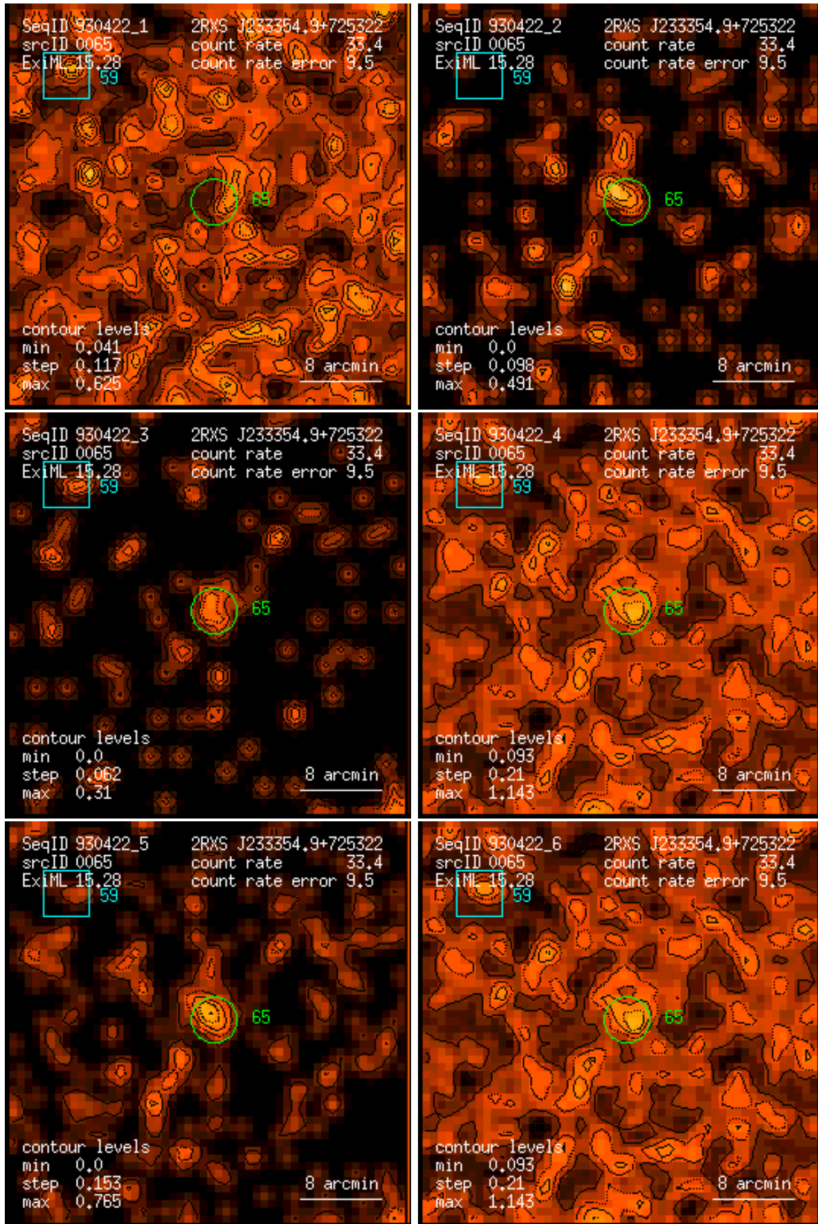
Figure 65: RASS 930422: detection 0065: band rate images, Gaussian filter: (1) PSPC channels 11 – 41, (2) 52 – 90, (3) 91 – 201, (4) 11 – 235, (5) 52 – 201, (6) 11 – 201. Broad band rates in counts/ks. Band rate contour levels in counts/ks/arcmin 2 .
