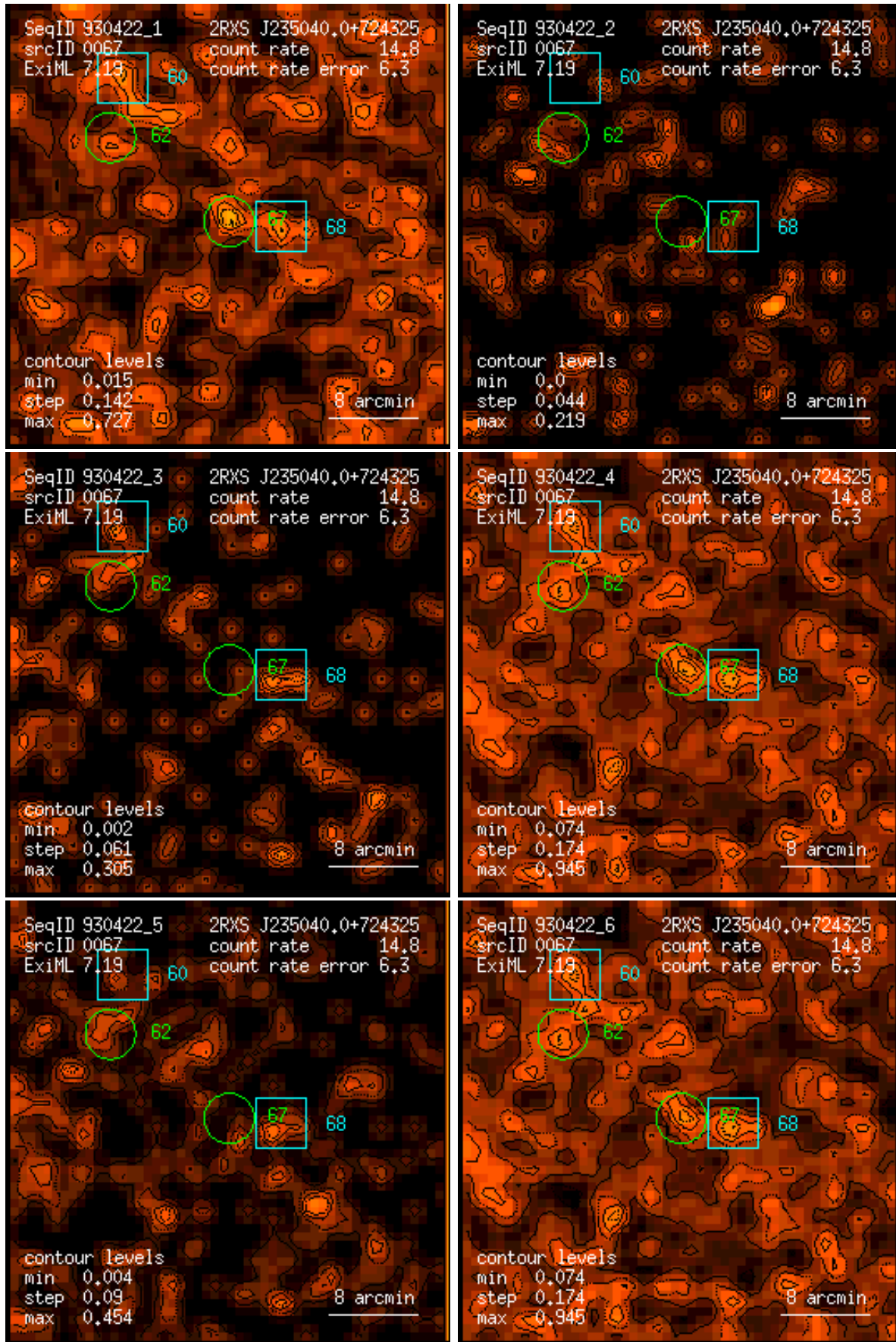
Figure 67: RASS 930422: detection 0067: band rate images, Gaussian filter: (1) PSPC channels 11 – 41, (2) 52 – 90, (3) 91 – 201, (4) 11 – 235, (5) 52 – 201, (6) 11 – 201. Broad band rates in counts/ks. Band rate contour levels in counts/ks/arcmin 2 .
