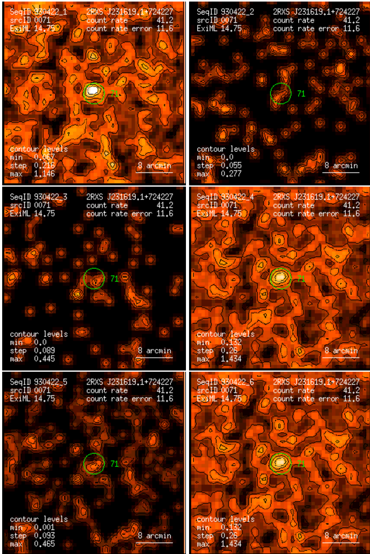
Figure 71: RASS 930422: detection 0071: band rate images, Gaussian filter: (1) PSPC channels 11 – 41, (2) 52 – 90, (3) 91 – 201, (4) 11 – 235, (5) 52 – 201, (6) 11 – 201. Broad band rates in counts/ks. Band rate contour levels in counts/ks/arcmin 2 .
