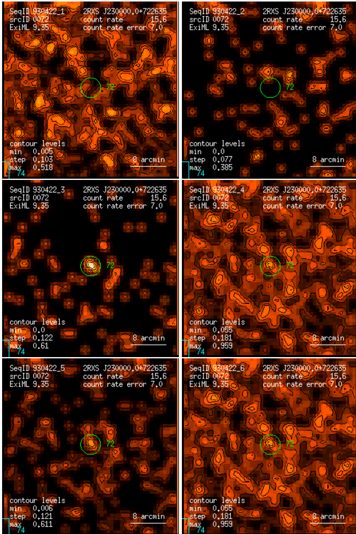
Figure 72: RASS 930422: detection 0072: band rate images, Gaussian filter: (1) PSPC channels 11 – 41, (2) 52 – 90, (3) 91 – 201, (4) 11 – 235, (5) 52 – 201, (6) 11 – 201. Broad band rates in counts/ks. Band rate contour levels in counts/ks/arcmin 2 .
