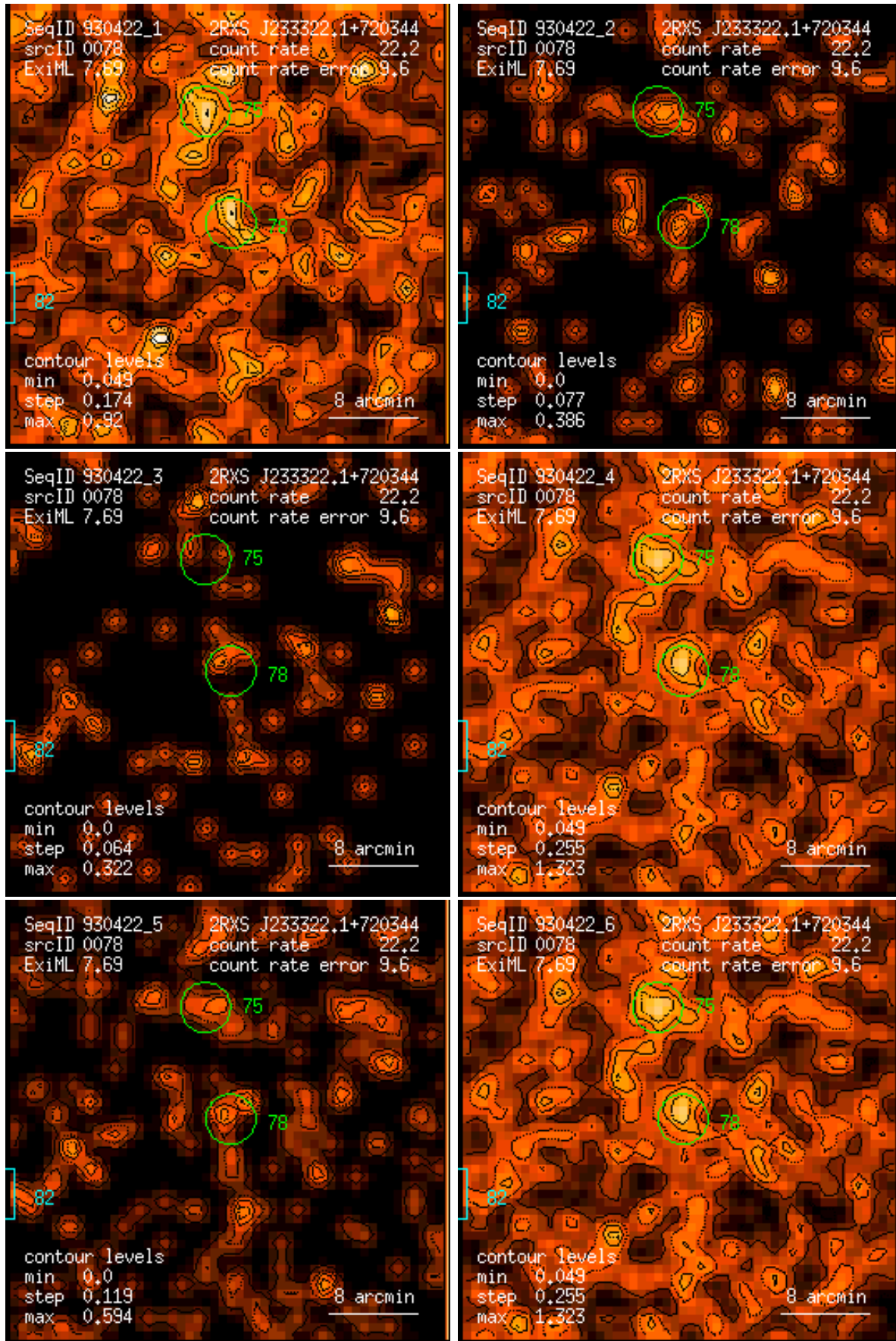
Figure 78: RASS 930422: detection 0078: band rate images, Gaussian filter: (1) PSPC channels 11 – 41, (2) 52 – 90, (3) 91 – 201, (4) 11 – 235, (5) 52 – 201, (6) 11 – 201. Broad band rates in counts/ks. Band rate contour levels in counts/ks/arcmin 2 .
