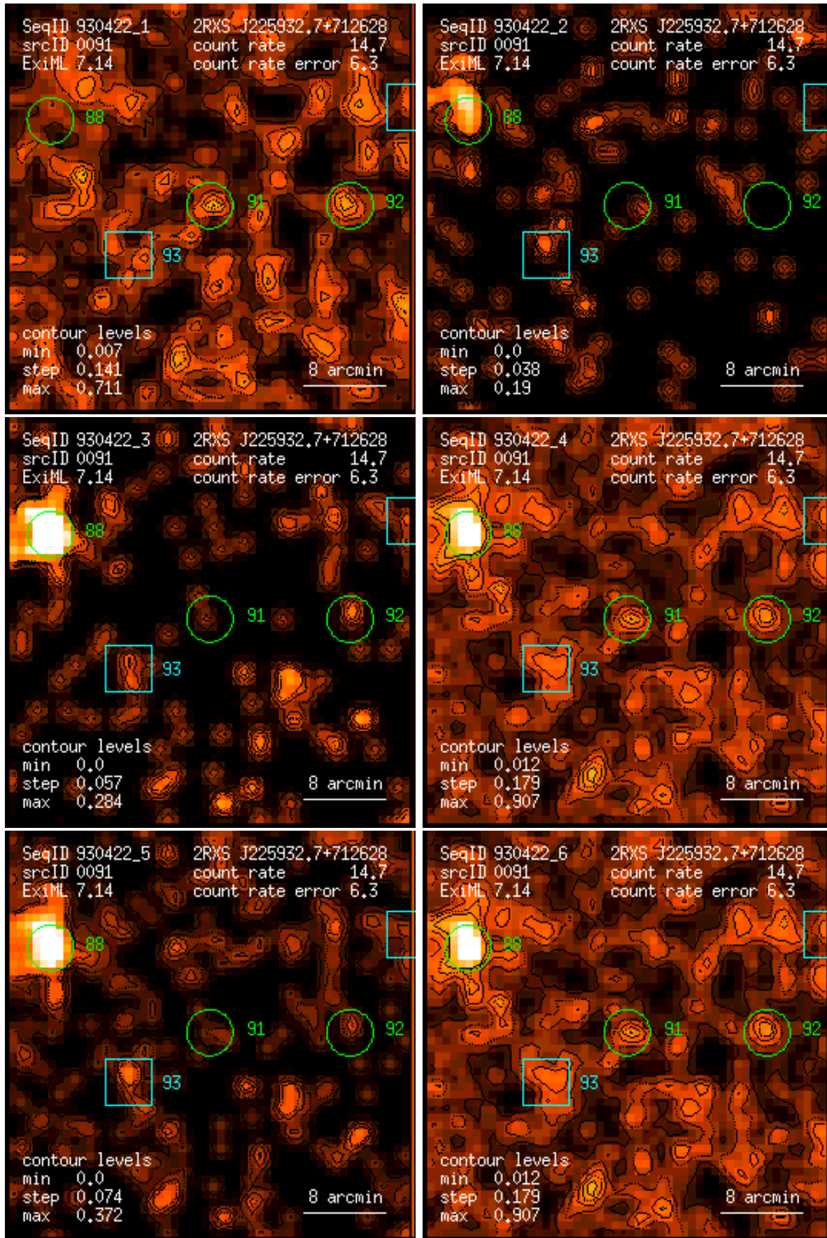
Figure 91: RASS 930422: detection 0091: band rate images, Gaussian filter: (1) PSPC channels 11 – 41, (2) 52 – 90, (3) 91 – 201, (4) 11 – 235, (5) 52 – 201, (6) 11 – 201. Broad band rates in counts/ks. Band rate contour levels in counts/ks/arcmin 2 .
