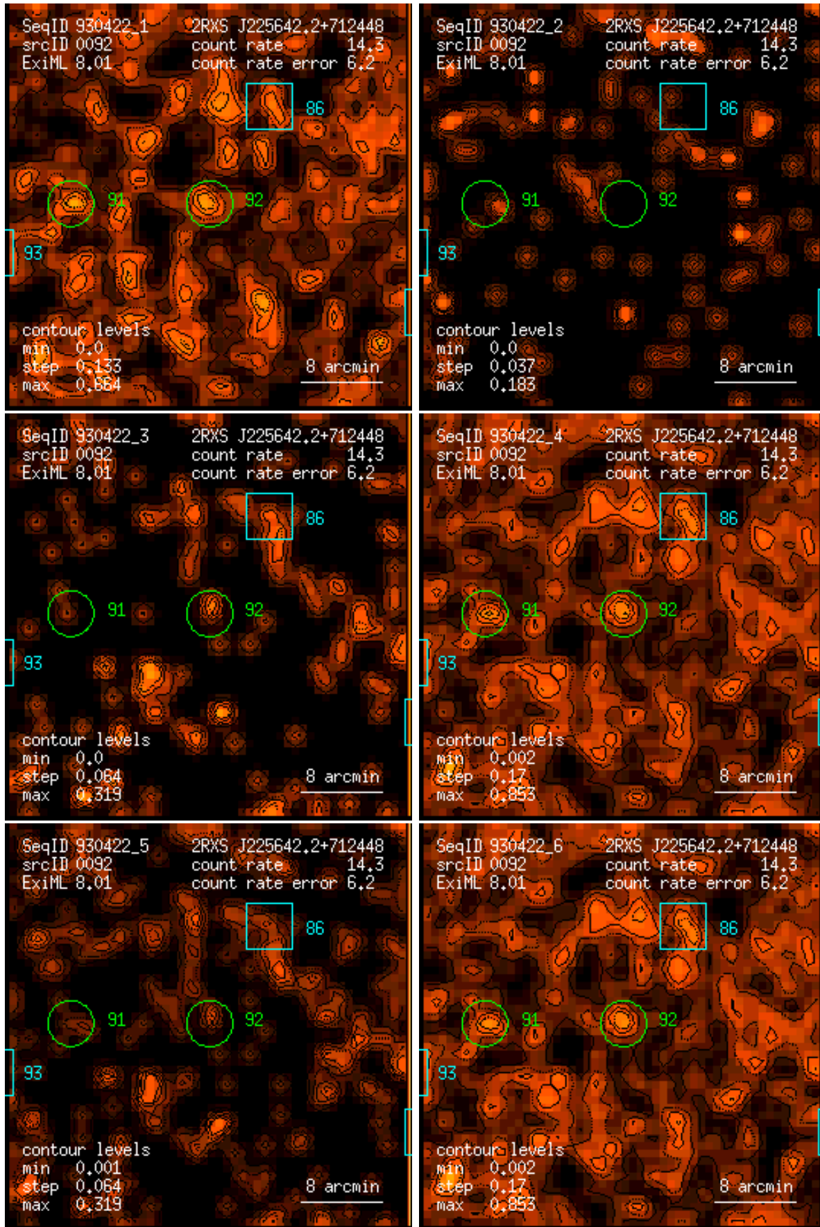
Figure 92: RASS 930422: detection 0092: band rate images, Gaussian filter: (1) PSPC channels 11 – 41, (2) 52 – 90, (3) 91 – 201, (4) 11 – 235, (5) 52 – 201, (6) 11 – 201. Broad band rates in counts/ks. Band rate contour levels in counts/ks/arcmin 2 .
