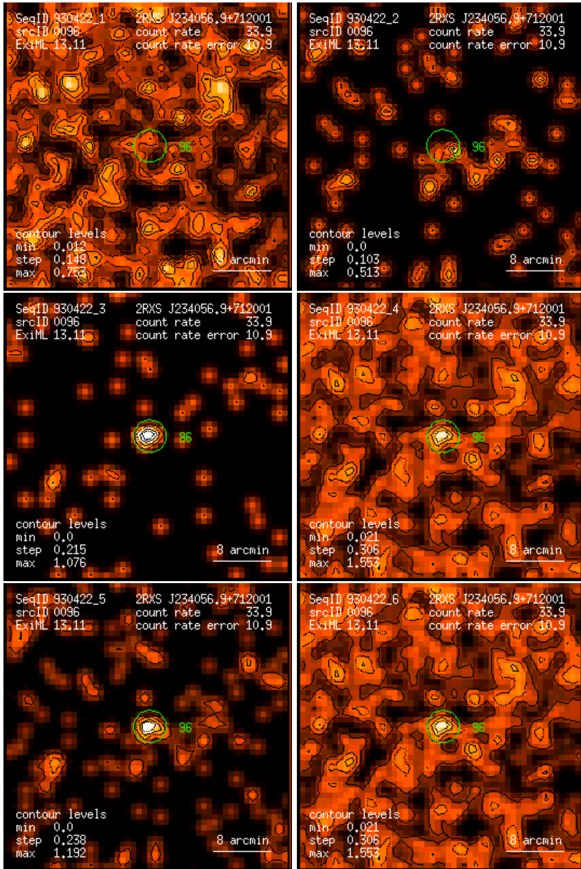
Figure 96: RASS 930422: detection 0096: band rate images, Gaussian filter: (1) PSPC channels 11 – 41, (2) 52 – 90, (3) 91 – 201, (4) 11 – 235, (5) 52 – 201, (6) 11 – 201. Broad band rates in counts/ks. Band rate contour levels in counts/ks/arcmin 2 .
