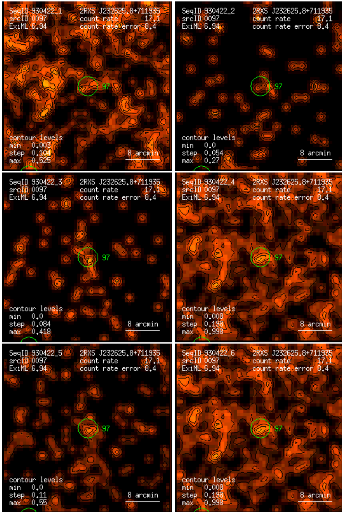
Figure 97: RASS 930422: detection 0097: band rate images, Gaussian filter: (1) PSPC channels 11 – 41, (2) 52 – 90, (3) 91 – 201, (4) 11 – 235, (5) 52 – 201, (6) 11 – 201. Broad band rates in counts/ks. Band rate contour levels in counts/ks/arcmin 2 .
