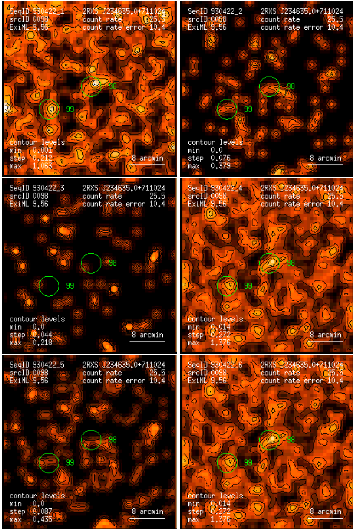
Figure 98: RASS 930422: detection 0098: band rate images, Gaussian filter: (1) PSPC channels 11 – 41, (2) 52 – 90, (3) 91 – 201, (4) 11 – 235, (5) 52 – 201, (6) 11 – 201. Broad band rates in counts/ks. Band rate contour levels in counts/ks/arcmin 2 .
