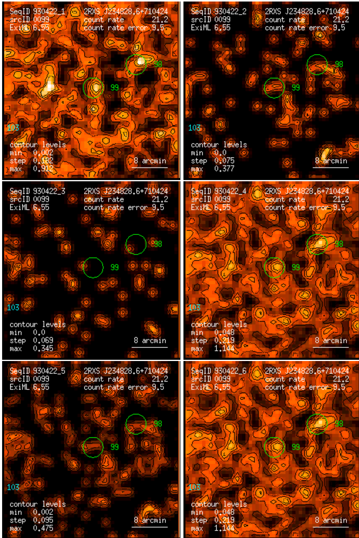
Figure 99: RASS 930422: detection 0099: band rate images, Gaussian filter: (1) PSPC channels 11 – 41, (2) 52 – 90, (3) 91 – 201, (4) 11 – 235, (5) 52 – 201, (6) 11 – 201. Broad band rates in counts/ks. Band rate contour levels in counts/ks/arcmin 2 .
