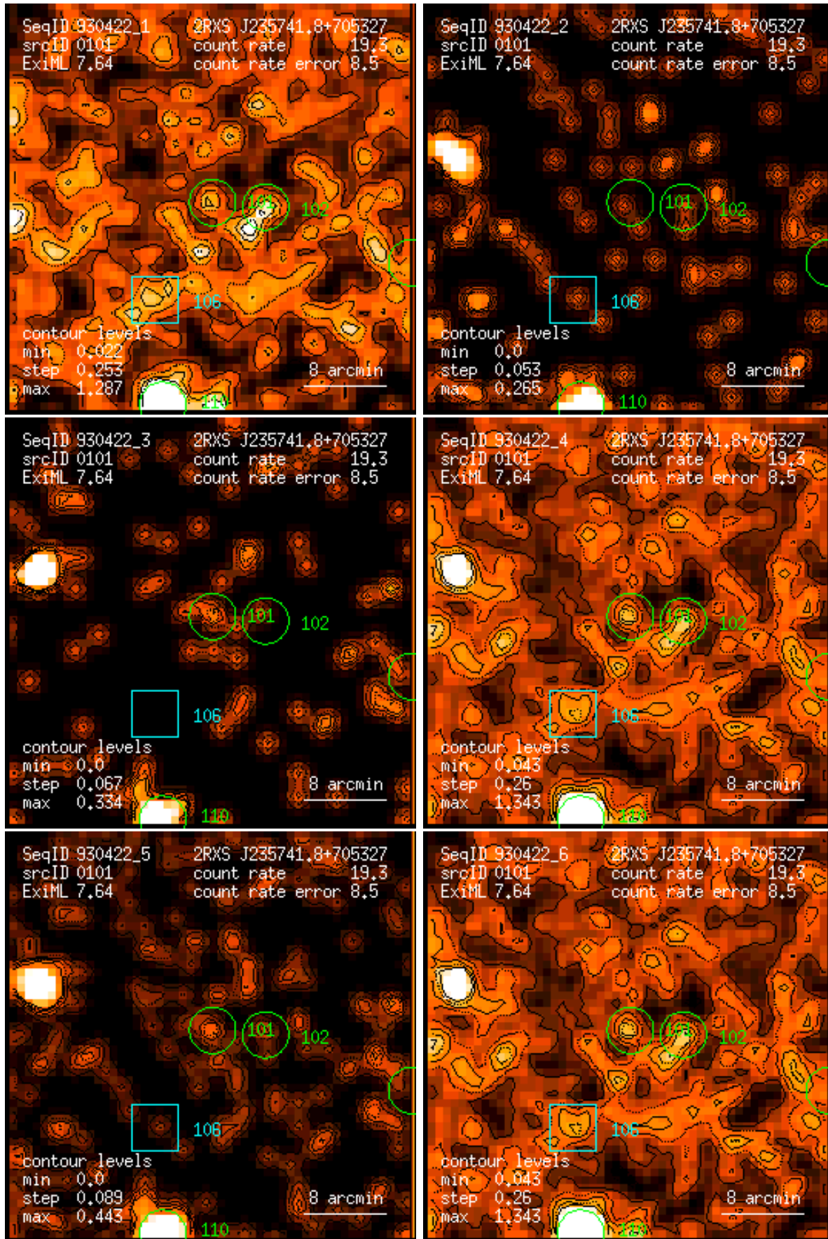
Figure 101: RASS 930422: detection 0101: band rate images, Gaussian filter: (1) PSPC channels 11 – 41, (2) 52 – 90, (3) 91 – 201, (4) 11 – 235, (5) 52 – 201, (6) 11 – 201. Broad band rates in counts/ks. Band rate contour levels in counts/ks/arcmin 2 .
