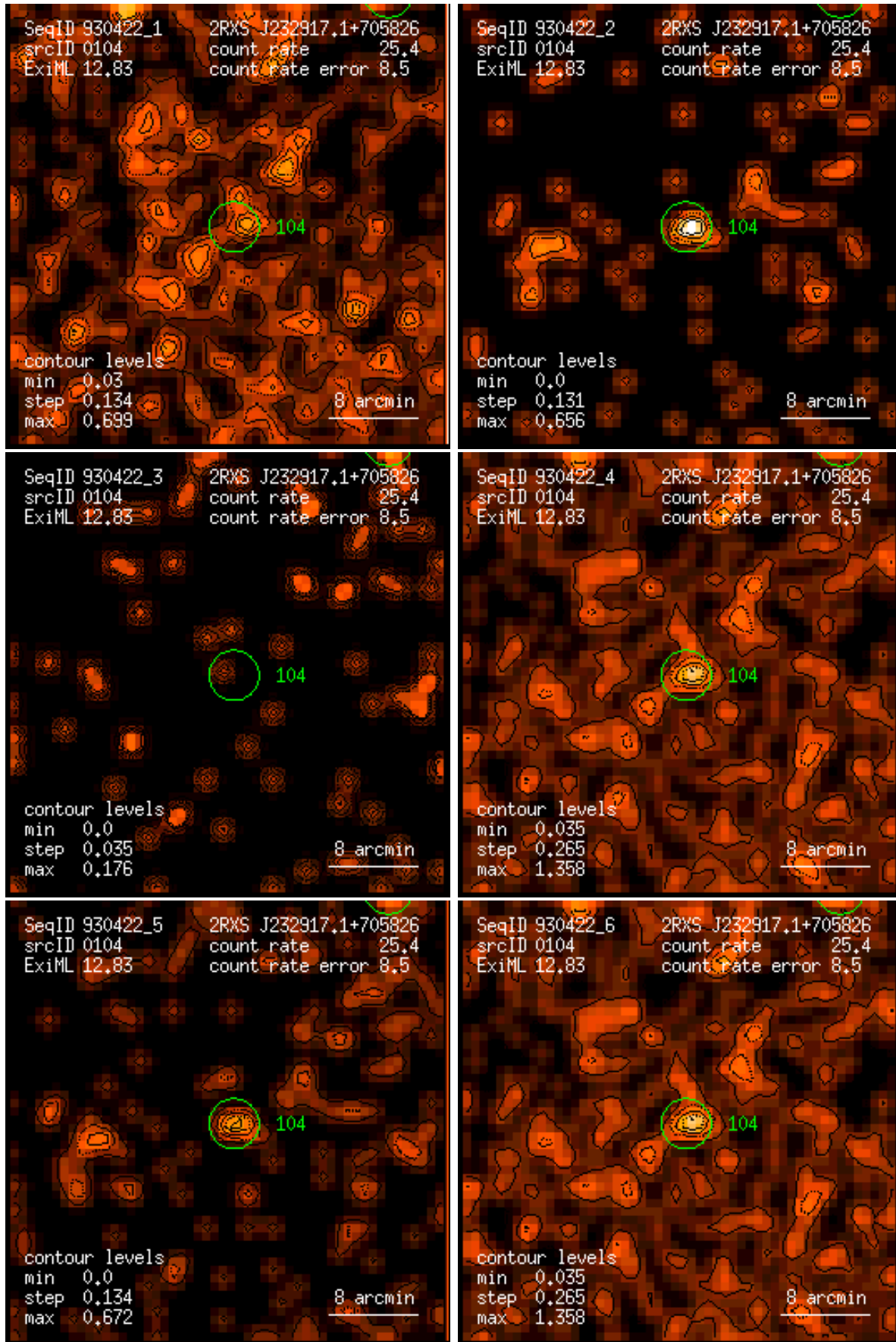
Figure 104: RASS 930422: detection 0104: band rate images, Gaussian filter: (1) PSPC channels 11 – 41, (2) 52 – 90, (3) 91 – 201, (4) 11 – 235, (5) 52 – 201, (6) 11 – 201. Broad band rates in counts/ks. Band rate contour levels in counts/ks/arcmin 2 .
