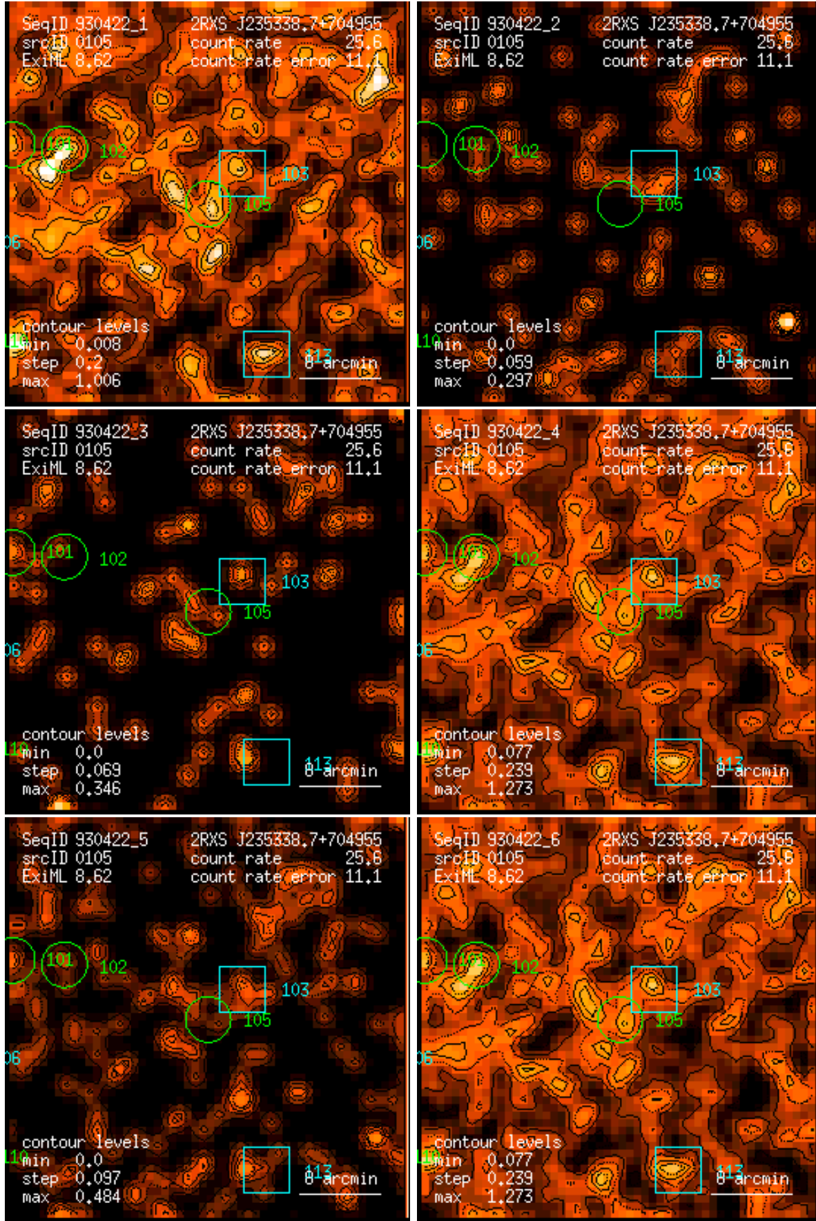
Figure 105: RASS 930422: detection 0105: band rate images, Gaussian filter: (1) PSPC channels 11 – 41, (2) 52 – 90, (3) 91 – 201, (4) 11 – 235, (5) 52 – 201, (6) 11 – 201. Broad band rates in counts/ks. Band rate contour levels in counts/ks/arcmin 2 .
