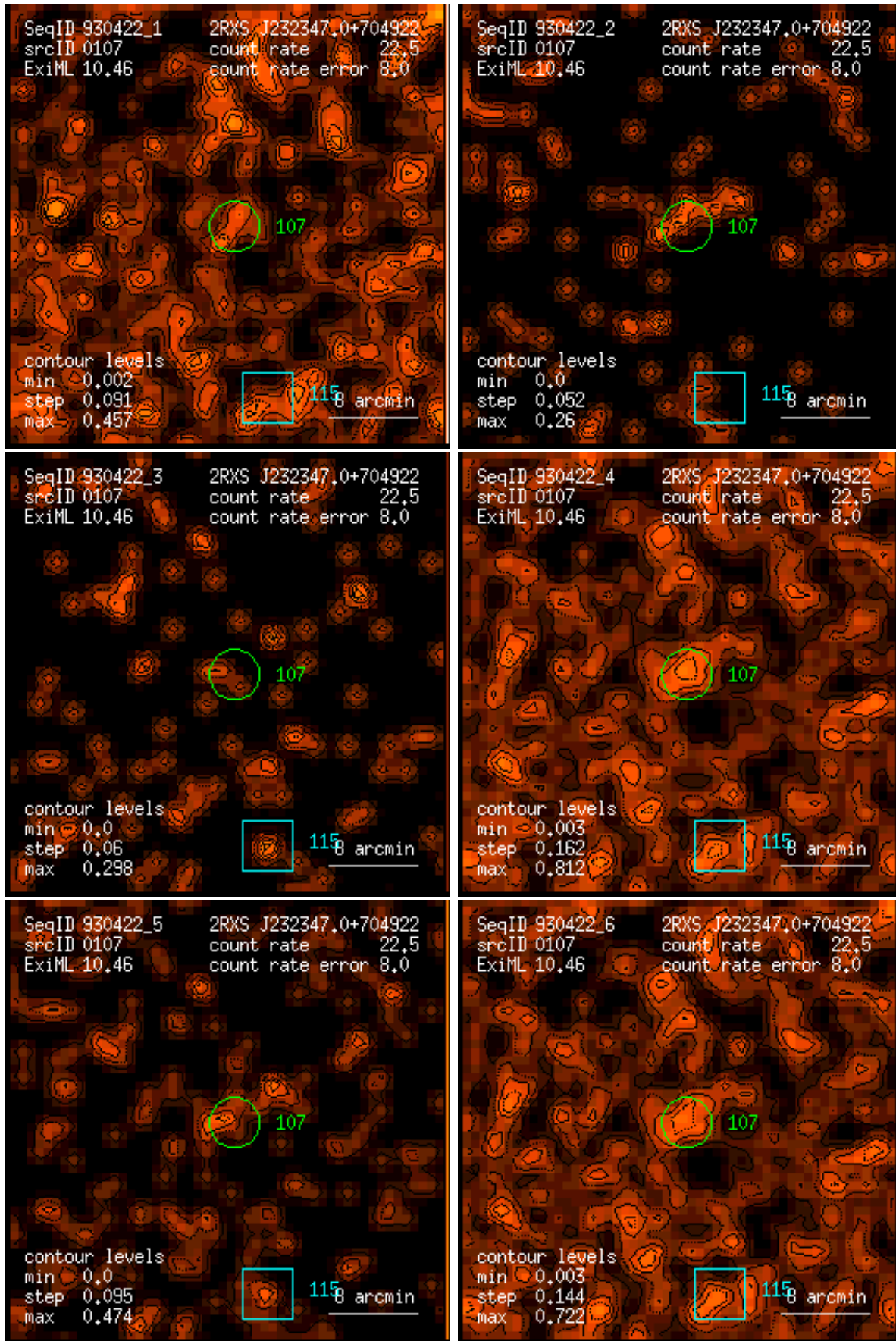
Figure 107: RASS 930422: detection 0107: band rate images, Gaussian filter: (1) PSPC channels 11 – 41, (2) 52 – 90, (3) 91 – 201, (4) 11 – 235, (5) 52 – 201, (6) 11 – 201. Broad band rates in counts/ks. Band rate contour levels in counts/ks/arcmin 2 .
