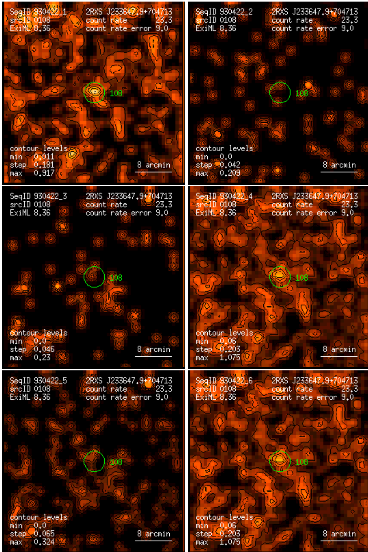
Figure 108: RASS 930422: detection 0108: band rate images, Gaussian filter: (1) PSPC channels 11 – 41, (2) 52 – 90, (3) 91 – 201, (4) 11 – 235, (5) 52 – 201, (6) 11 – 201. Broad band rates in counts/ks. Band rate contour levels in counts/ks/arcmin 2 .
