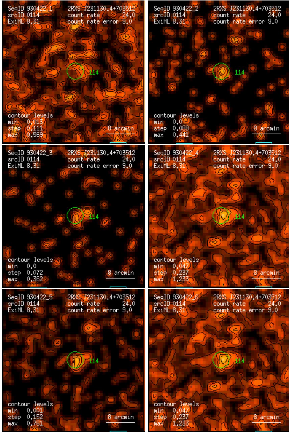
Figure 114: RASS 930422: detection 0114: band rate images, Gaussian filter: (1) PSPC channels 11 – 41, (2) 52 – 90, (3) 91 – 201, (4) 11 – 235, (5) 52 – 201, (6) 11 – 201. Broad band rates in counts/ks. Band rate contour levels in counts/ks/arcmin 2 .
