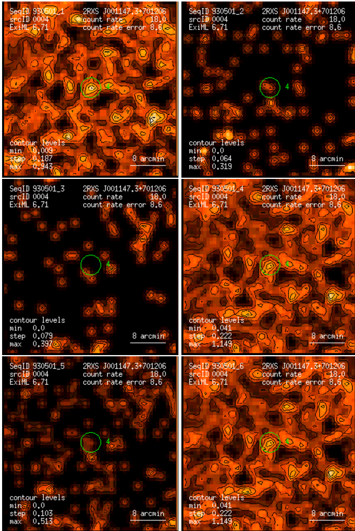
Figure 4: RASS 930501: detection 0004: band rate images, Gaussian filter: (1) PSPC channels 11 – 41, (2) 52 – 90, (3) 91 – 201, (4) 11 – 235, (5) 52 – 201, (6) 11 – 201. Broad band rates in counts/ks. Band rate contour levels in counts/ks/arcmin 2 .
