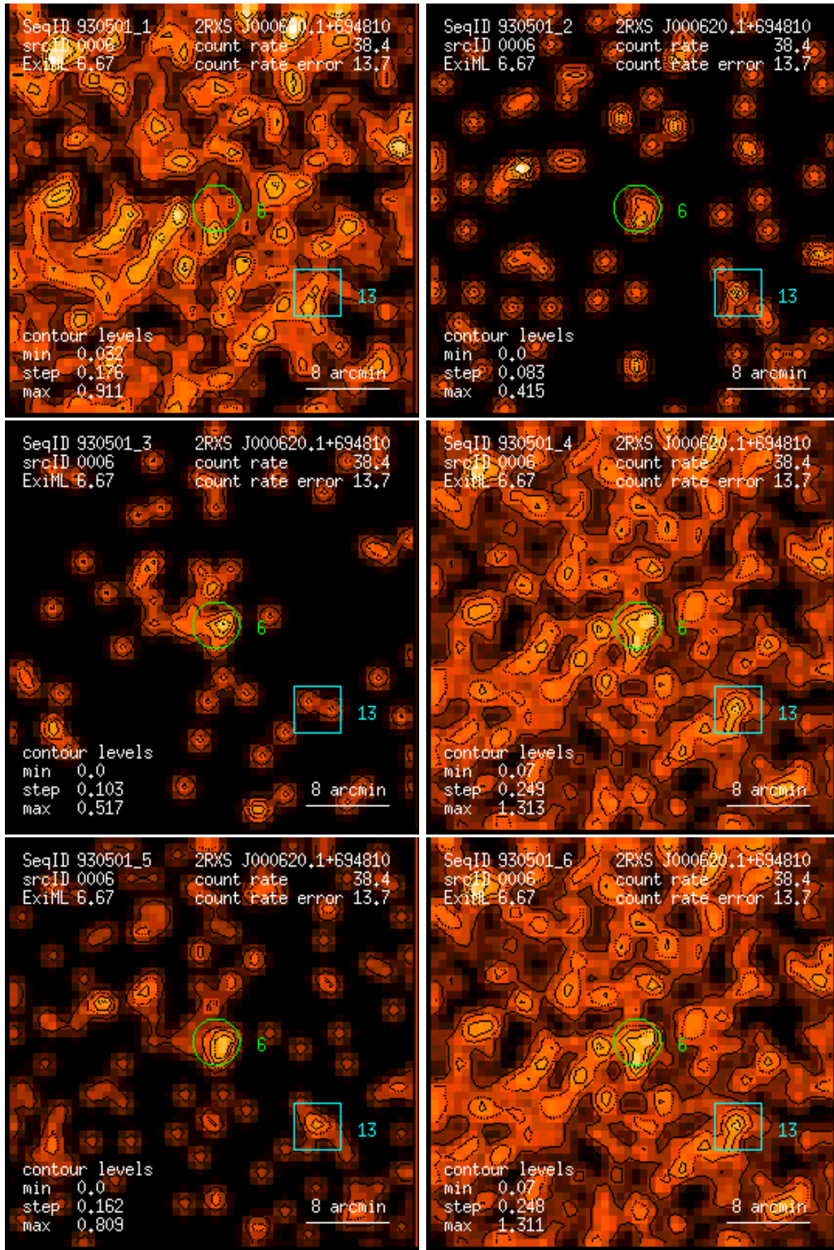
Figure 6: RASS 930501: detection 0006: band rate images, Gaussian filter: (1) PSPC channels 11 – 41, (2) 52 – 90, (3) 91 – 201, (4) 11 – 235, (5) 52 – 201, (6) 11 – 201. Broad band rates in counts/ks. Band rate contour levels in counts/ks/arcmin 2 .
