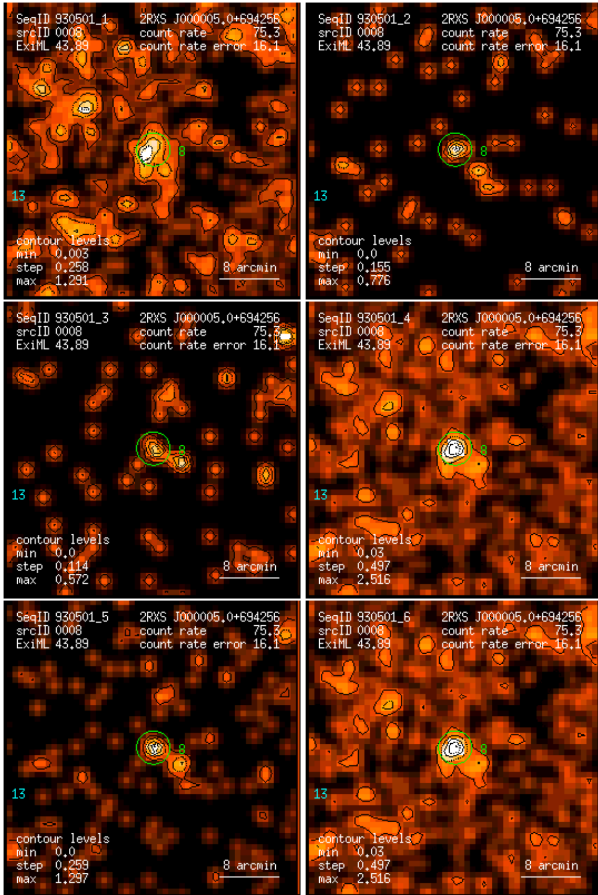
Figure 8: RASS 930501: detection 0008: band rate images, Gaussian filter: (1) PSPC channels 11 – 41, (2) 52 – 90, (3) 91 – 201, (4) 11 – 235, (5) 52 – 201, (6) 11 – 201. Broad band rates in counts/ks. Band rate contour levels in counts/ks/arcmin 2 .
