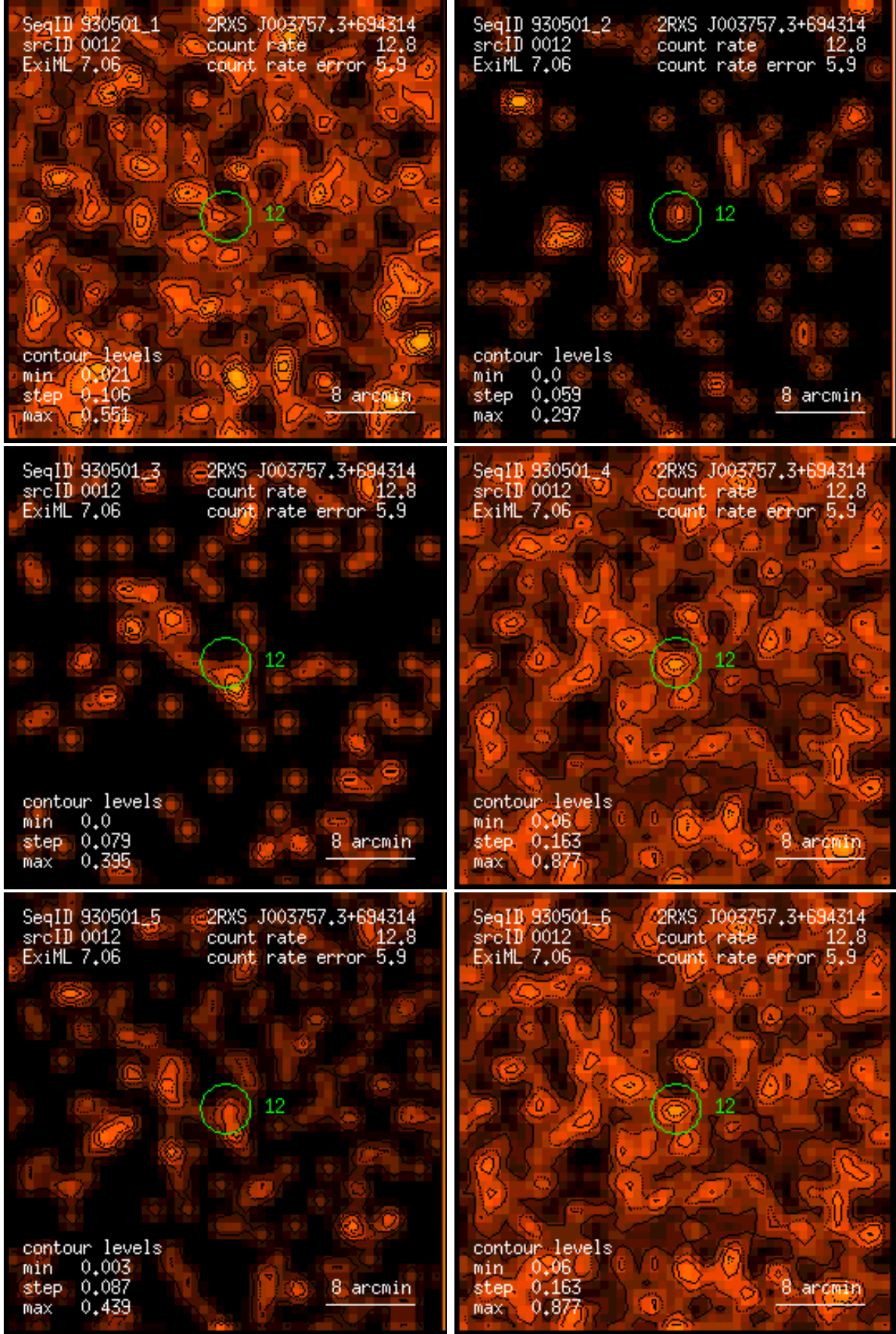
Figure 12: RASS 930501: detection 0012: band rate images, Gaussian filter: (1) PSPC channels 11 – 41, (2) 52 – 90, (3) 91 – 201, (4) 11 – 235, (5) 52 – 201, (6) 11 – 201. Broad band rates in counts/ks. Band rate contour levels in counts/ks/arcmin 2 .
