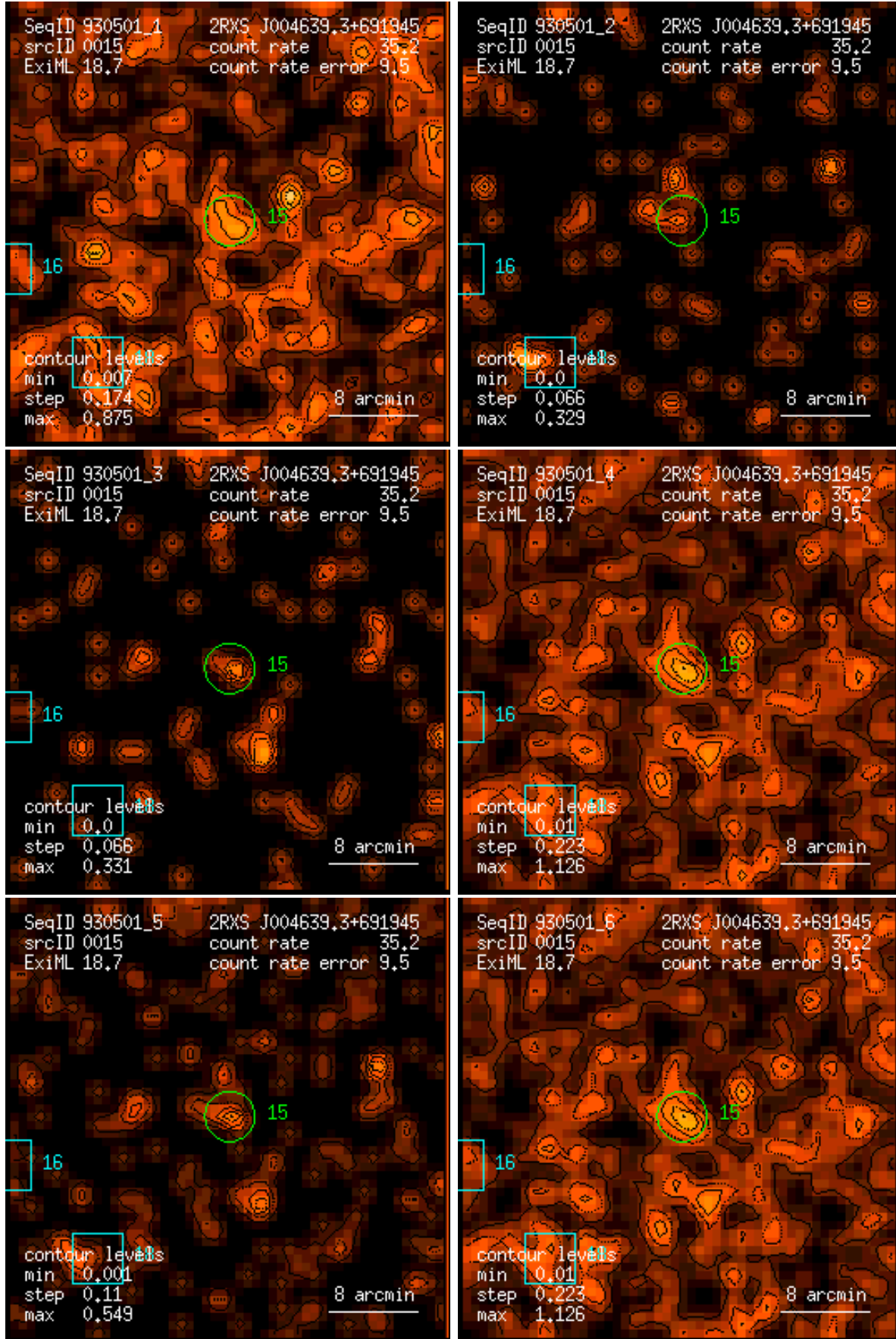
Figure 15: RASS 930501: detection 0015: band rate images, Gaussian filter: (1) PSPC channels 11 – 41, (2) 52 – 90, (3) 91 – 201, (4) 11 – 235, (5) 52 – 201, (6) 11 – 201. Broad band rates in counts/ks. Band rate contour levels in counts/ks/arcmin 2 .
