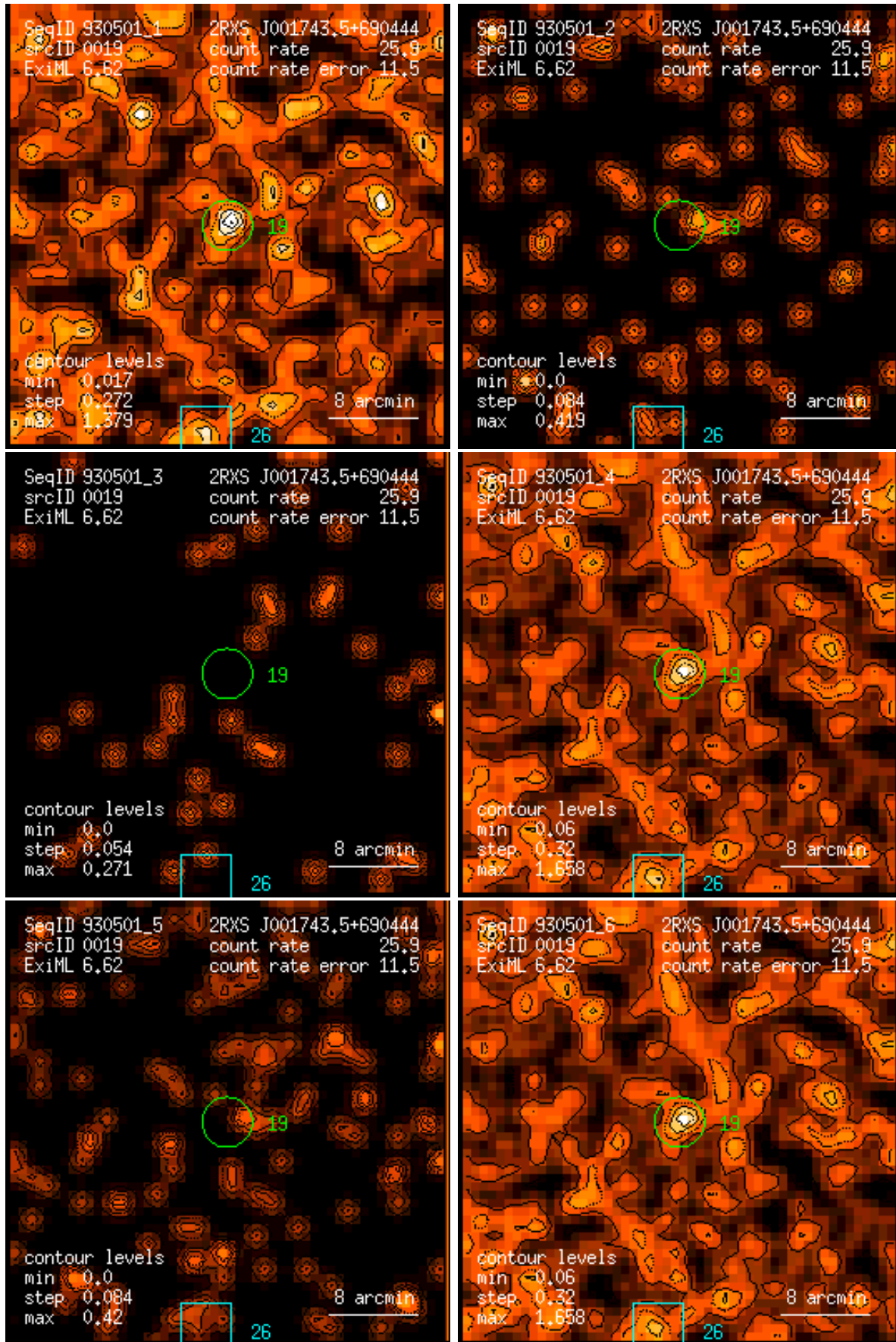
Figure 19: RASS 930501: detection 0019: band rate images, Gaussian filter: (1) PSPC channels 11 – 41, (2) 52 – 90, (3) 91 – 201, (4) 11 – 235, (5) 52 – 201, (6) 11 – 201. Broad band rates in counts/ks. Band rate contour levels in counts/ks/arcmin 2 .
