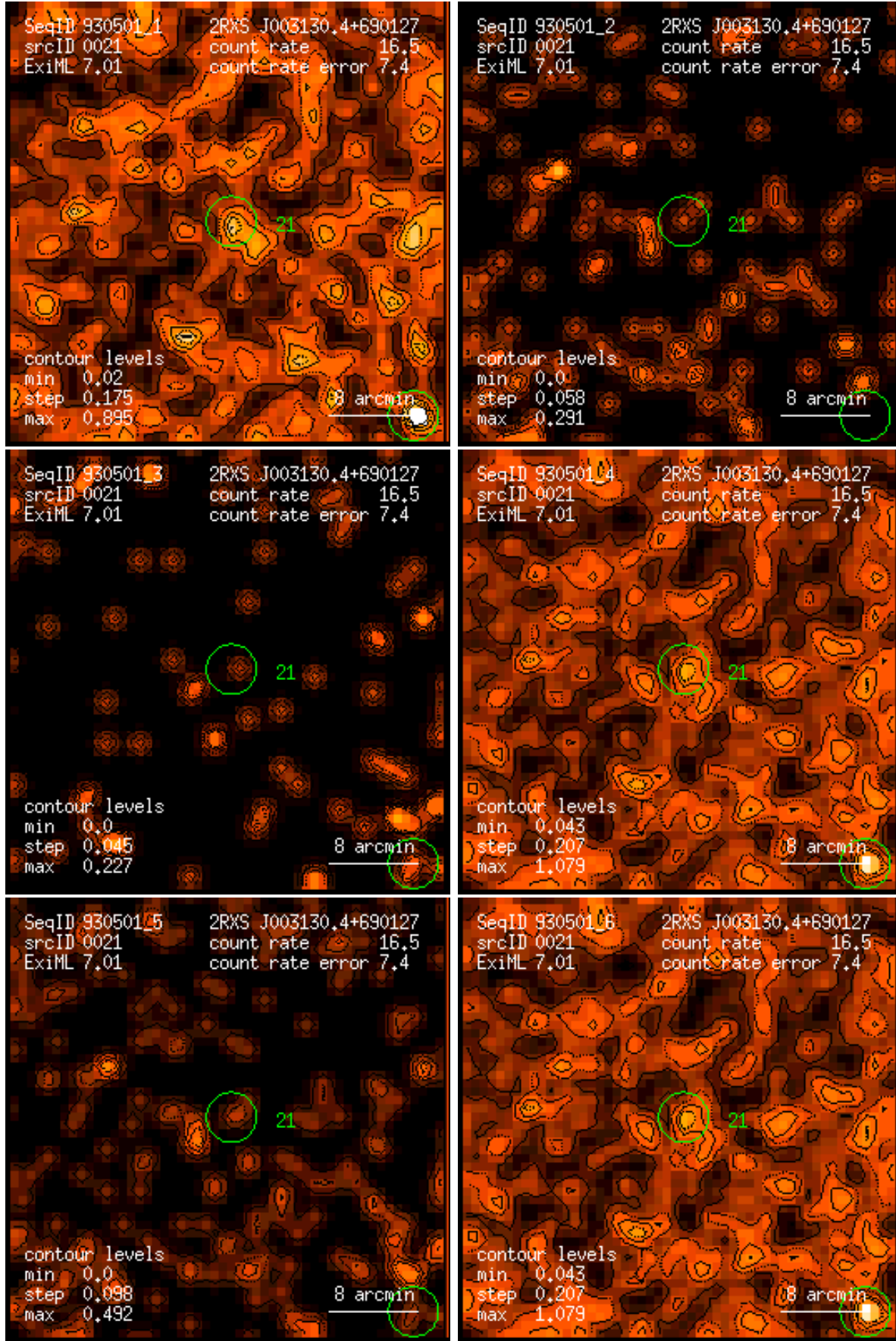
Figure 21: RASS 930501: detection 0021: band rate images, Gaussian filter: (1) PSPC channels 11 – 41, (2) 52 – 90, (3) 91 – 201, (4) 11 – 235, (5) 52 – 201, (6) 11 – 201. Broad band rates in counts/ks. Band rate contour levels in counts/ks/arcmin 2 .
