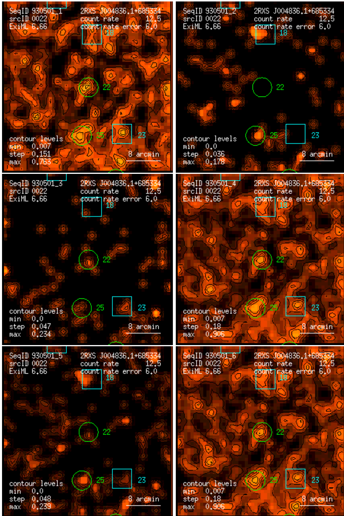
Figure 22: RASS 930501: detection 0022: band rate images, Gaussian filter: (1) PSPC channels 11 – 41, (2) 52 – 90, (3) 91 – 201, (4) 11 – 235, (5) 52 – 201, (6) 11 – 201. Broad band rates in counts/ks. Band rate contour levels in counts/ks/arcmin 2 .
