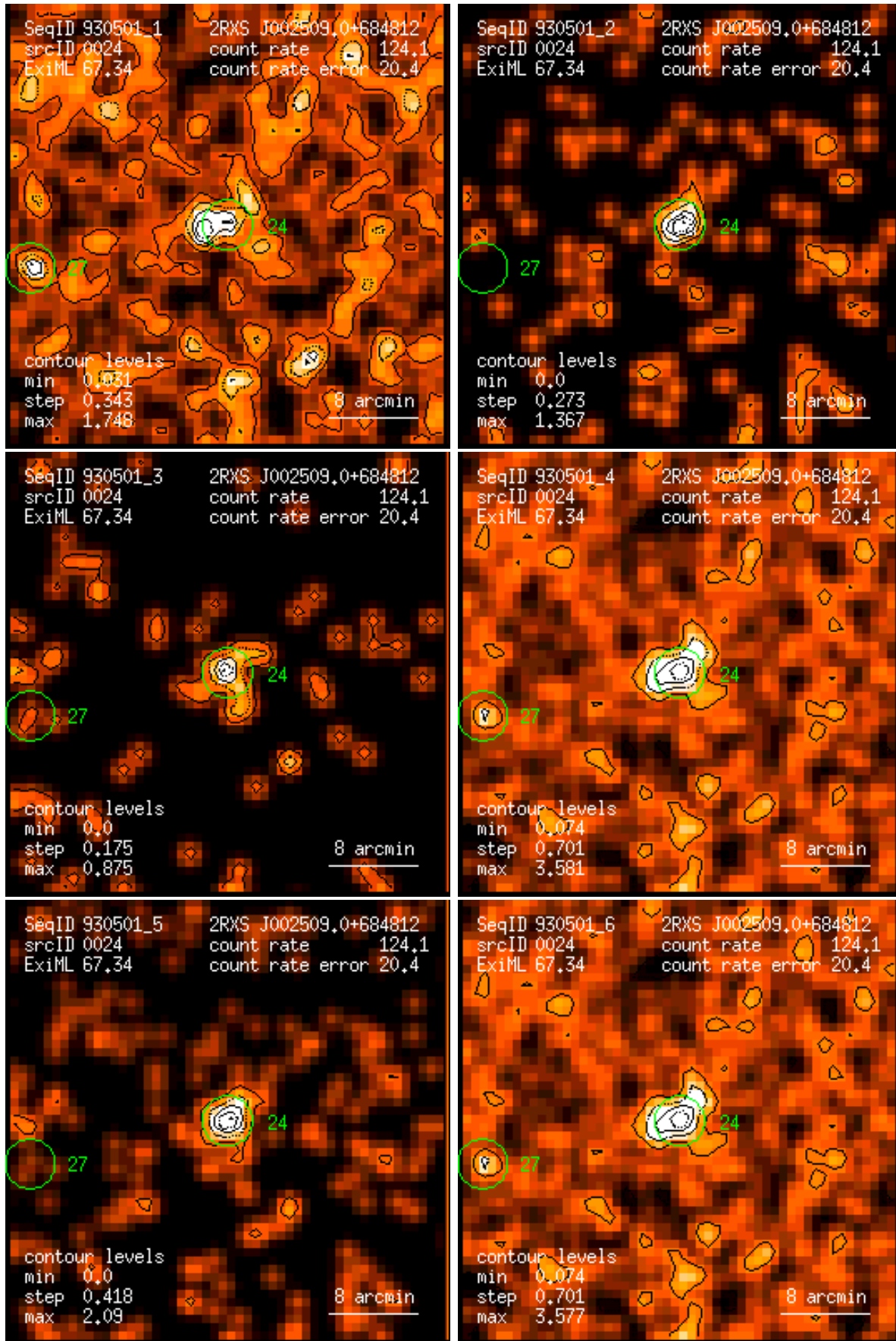
Figure 24: RASS 930501: detection 0024: band rate images, Gaussian filter: (1) PSPC channels 11 – 41, (2) 52 – 90, (3) 91 – 201, (4) 11 – 235, (5) 52 – 201, (6) 11 – 201. Broad band rates in counts/ks. Band rate contour levels in counts/ks/arcmin 2 .
