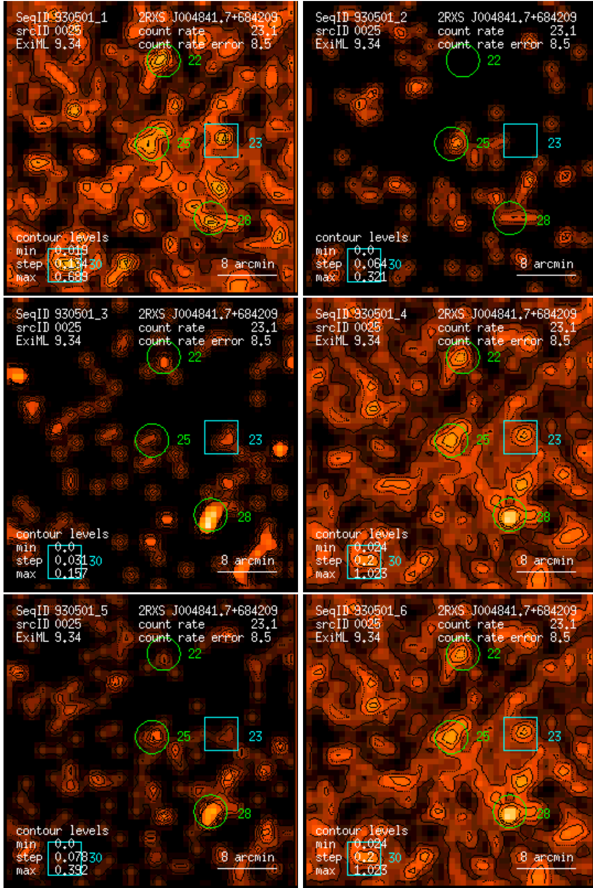
Figure 25: RASS 930501: detection 0025: band rate images, Gaussian filter: (1) PSPC channels 11 – 41, (2) 52 – 90, (3) 91 – 201, (4) 11 – 235, (5) 52 – 201, (6) 11 – 201. Broad band rates in counts/ks. Band rate contour levels in counts/ks/arcmin 2 .
