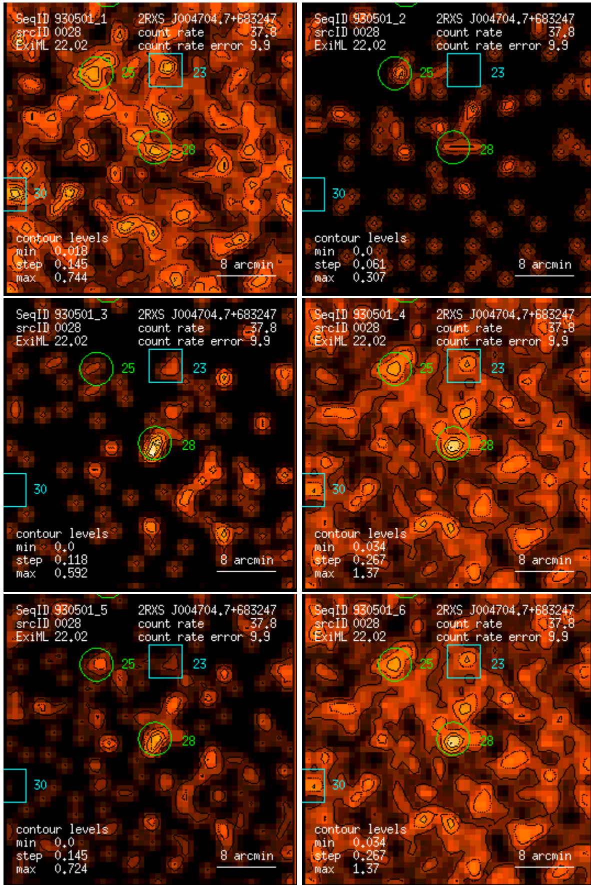
Figure 28: RASS 930501: detection 0028: band rate images, Gaussian filter: (1) PSPC channels 11 – 41, (2) 52 – 90, (3) 91 – 201, (4) 11 – 235, (5) 52 – 201, (6) 11 – 201. Broad band rates in counts/ks. Band rate contour levels in counts/ks/arcmin 2 .
