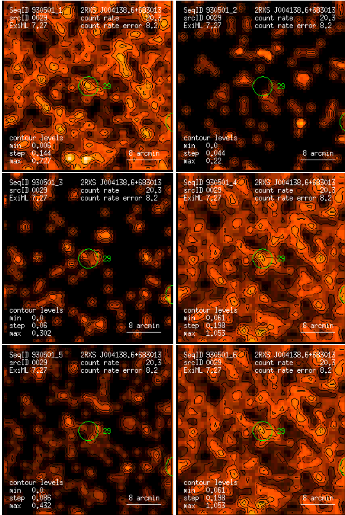
Figure 29: RASS 930501: detection 0029: band rate images, Gaussian filter: (1) PSPC channels 11 – 41, (2) 52 – 90, (3) 91 – 201, (4) 11 – 235, (5) 52 – 201, (6) 11 – 201. Broad band rates in counts/ks. Band rate contour levels in counts/ks/arcmin 2 .
