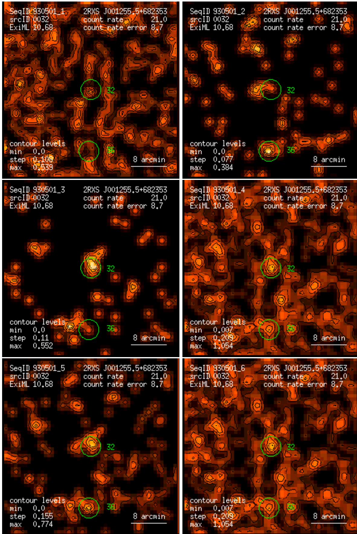
Figure 32: RASS 930501: detection 0032: band rate images, Gaussian filter: (1) PSPC channels 11 – 41, (2) 52 – 90, (3) 91 – 201, (4) 11 – 235, (5) 52 – 201, (6) 11 – 201. Broad band rates in counts/ks. Band rate contour levels in counts/ks/arcmin 2 .
