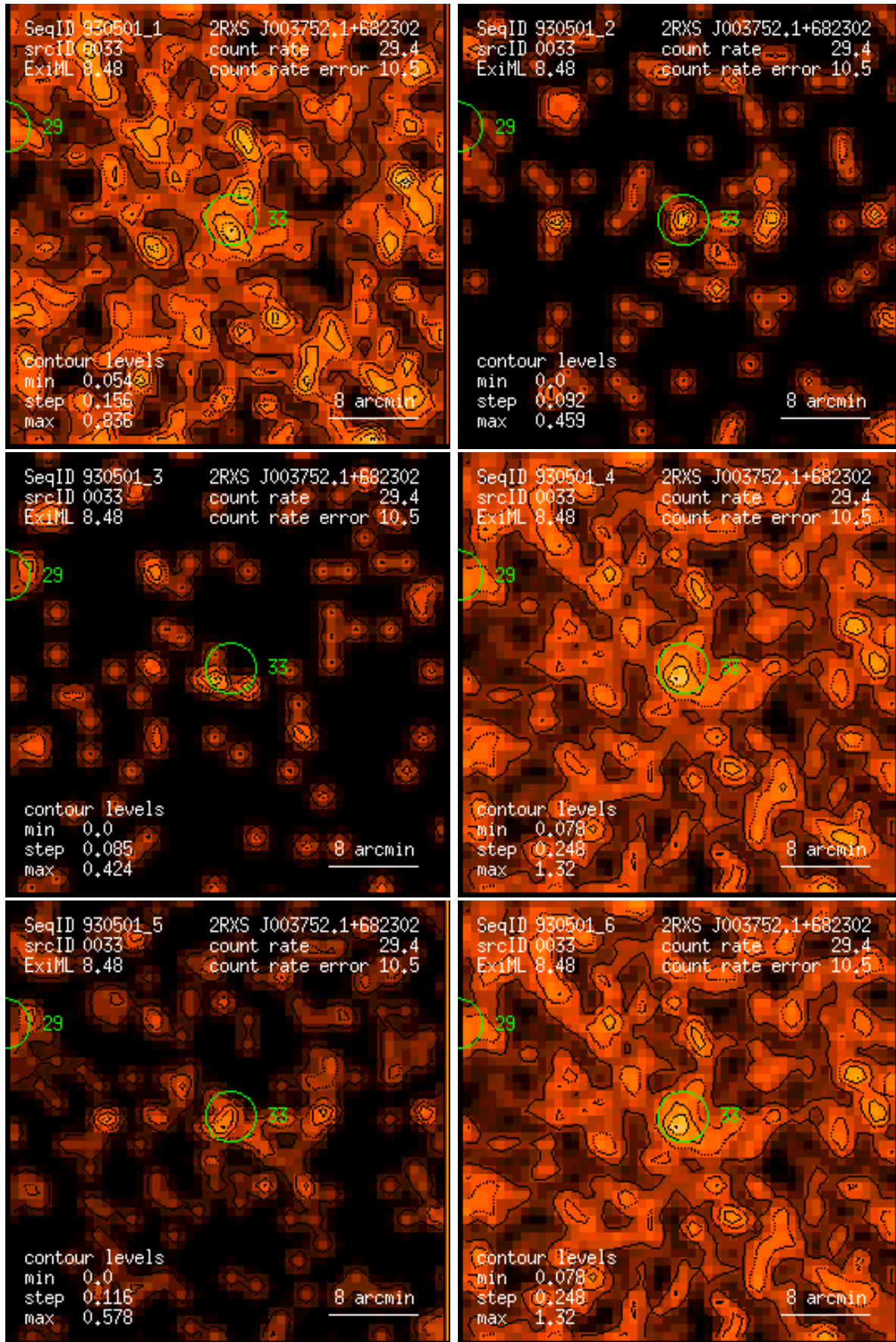
Figure 33: RASS 930501: detection 0033: band rate images, Gaussian filter: (1) PSPC channels 11 – 41, (2) 52 – 90, (3) 91 – 201, (4) 11 – 235, (5) 52 – 201, (6) 11 – 201. Broad band rates in counts/ks. Band rate contour levels in counts/ks/arcmin 2 .
