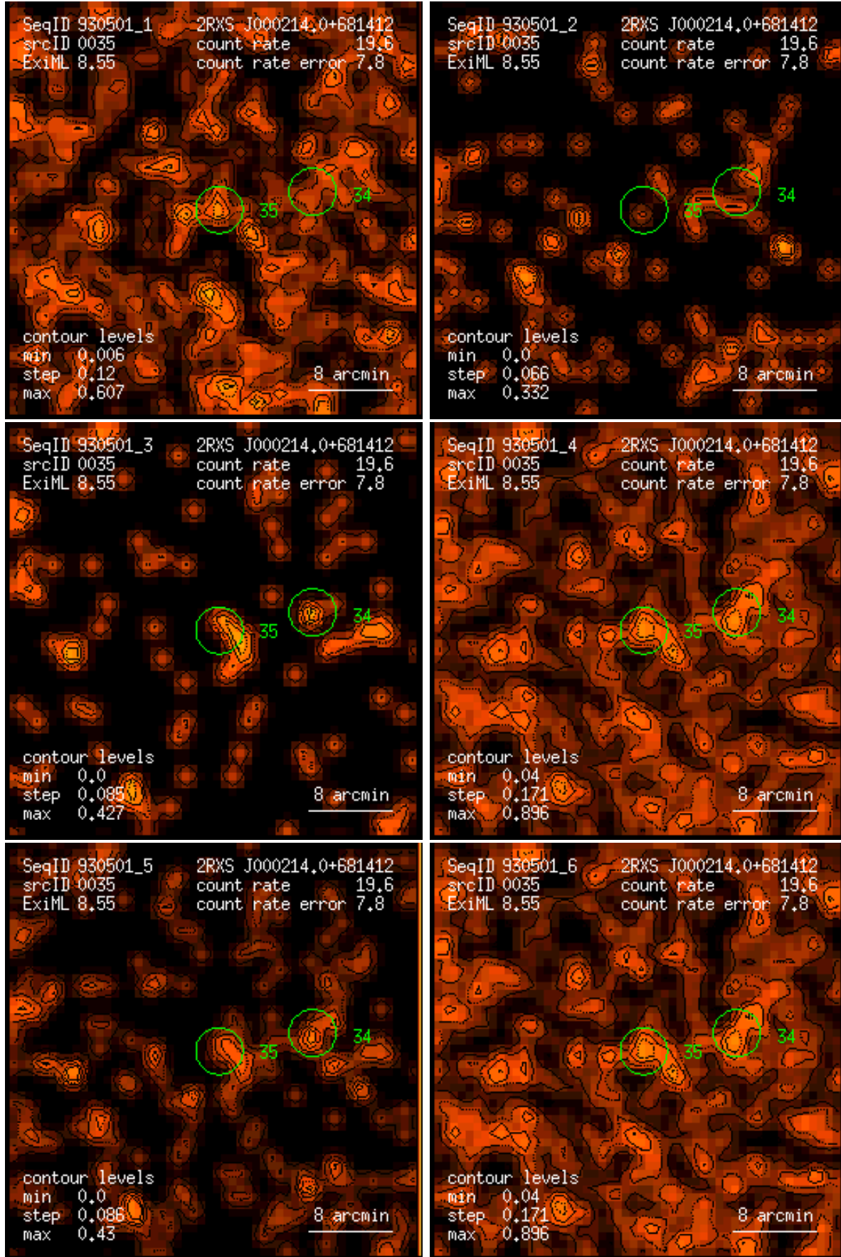
Figure 35: RASS 930501: detection 0035: band rate images, Gaussian filter: (1) PSPC channels 11 – 41, (2) 52 – 90, (3) 91 – 201, (4) 11 – 235, (5) 52 – 201, (6) 11 – 201. Broad band rates in counts/ks. Band rate contour levels in counts/ks/arcmin 2 .
