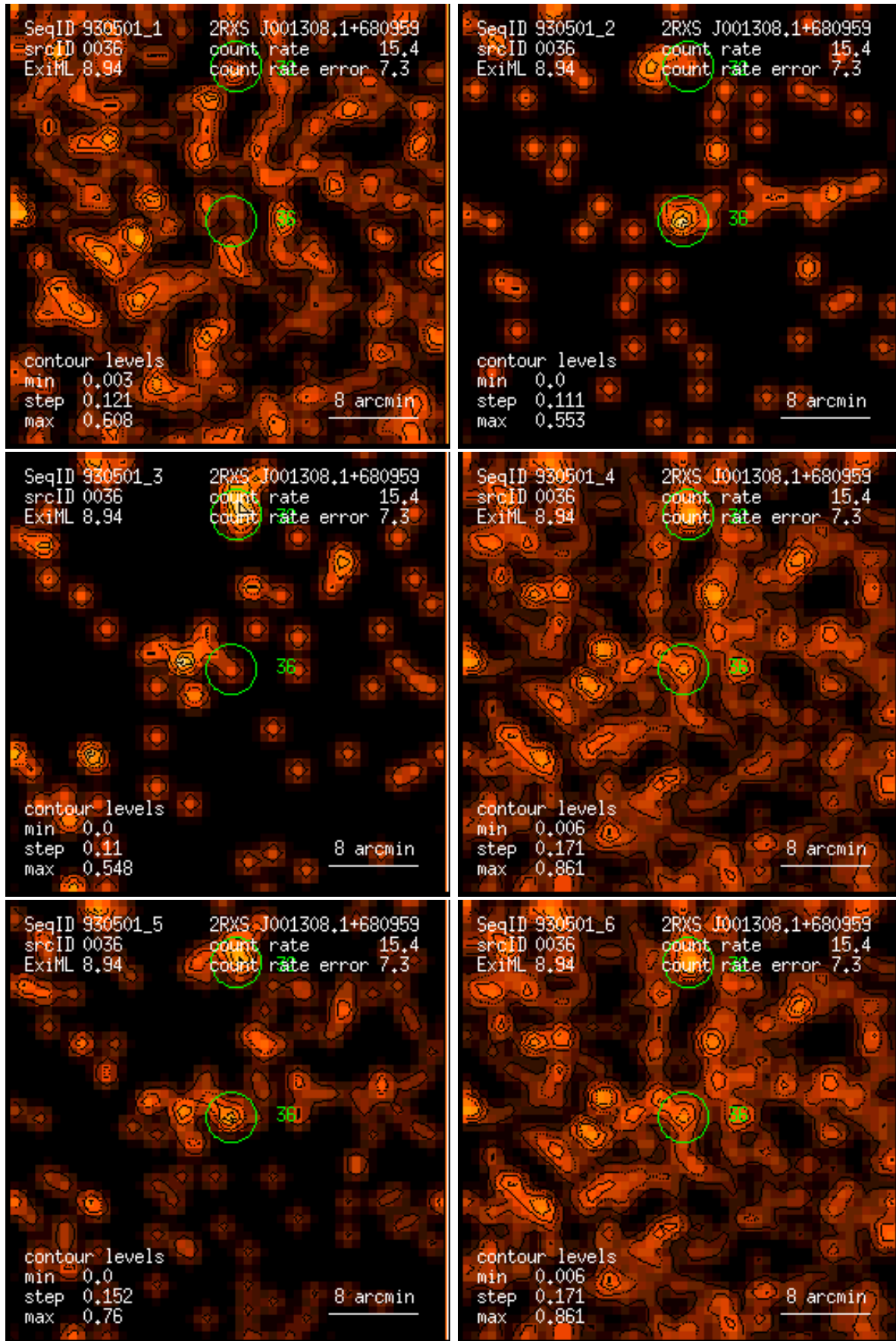
Figure 36: RASS 930501: detection 0036: band rate images, Gaussian filter: (1) PSPC channels 11 – 41, (2) 52 – 90, (3) 91 – 201, (4) 11 – 235, (5) 52 – 201, (6) 11 – 201. Broad band rates in counts/ks. Band rate contour levels in counts/ks/arcmin 2 .
