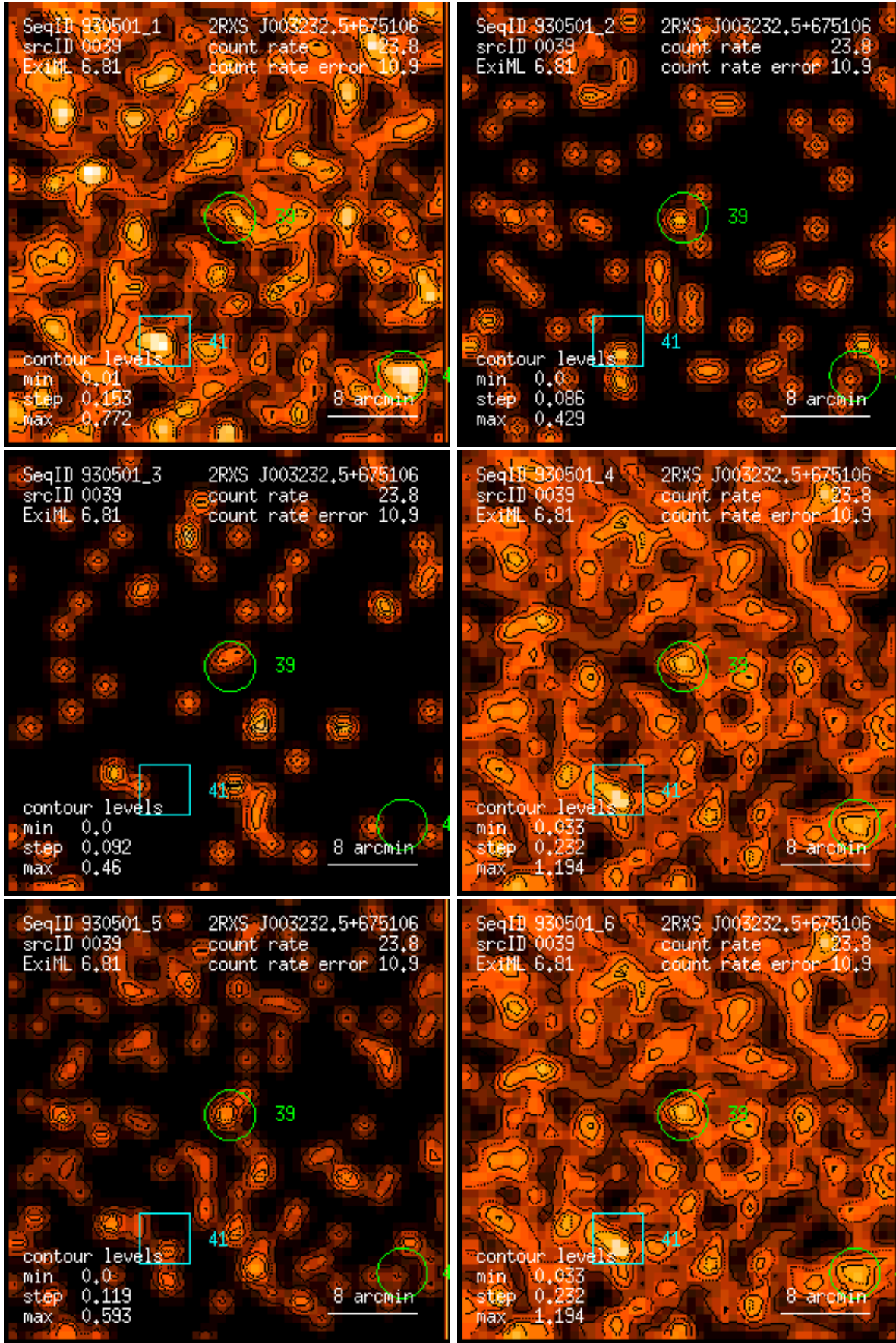
Figure 39: RASS 930501: detection 0039: band rate images, Gaussian filter: (1) PSPC channels 11 – 41, (2) 52 – 90, (3) 91 – 201, (4) 11 – 235, (5) 52 – 201, (6) 11 – 201. Broad band rates in counts/ks. Band rate contour levels in counts/ks/arcmin 2 .
