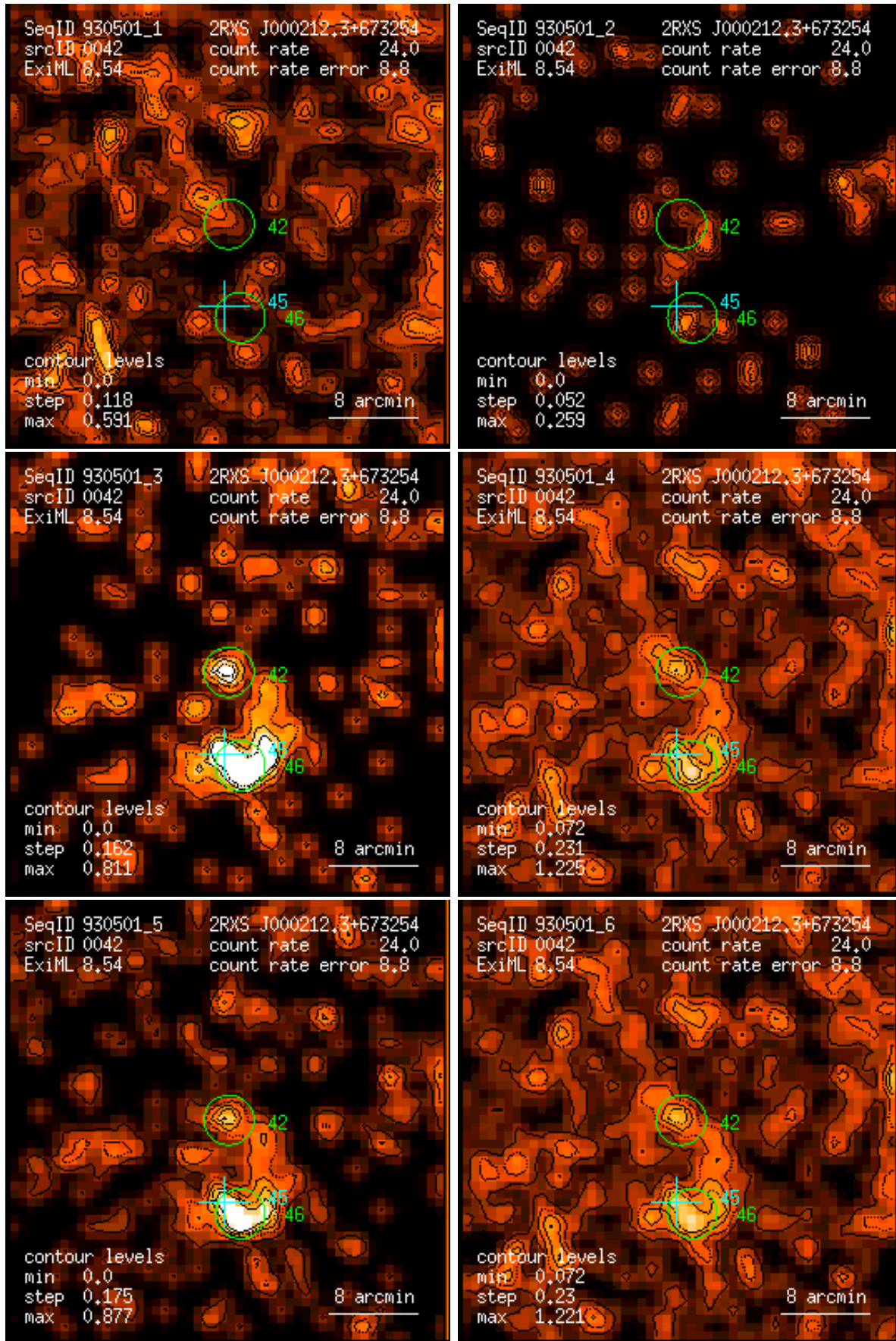
Figure 42: RASS 930501: detection 0042: band rate images, Gaussian filter: (1) PSPC channels 11 – 41, (2) 52 – 90, (3) 91 – 201, (4) 11 – 235, (5) 52 – 201, (6) 11 – 201. Broad band rates in counts/ks. Band rate contour levels in counts/ks/arcmin 2 .
