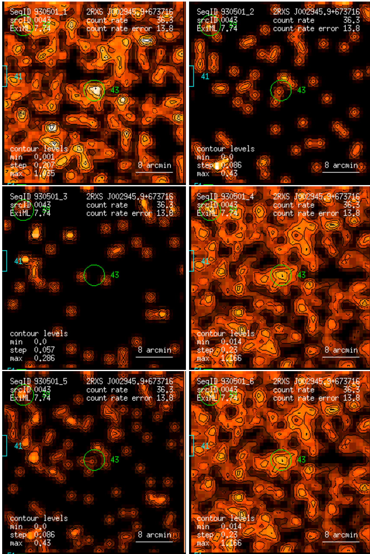
Figure 43: RASS 930501: detection 0043: band rate images, Gaussian filter: (1) PSPC channels 11 – 41, (2) 52 – 90, (3) 91 – 201, (4) 11 – 235, (5) 52 – 201, (6) 11 – 201. Broad band rates in counts/ks. Band rate contour levels in counts/ks/arcmin 2 .
